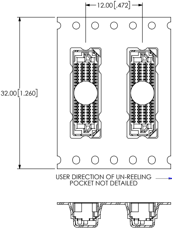
PACKAGING VIEW
