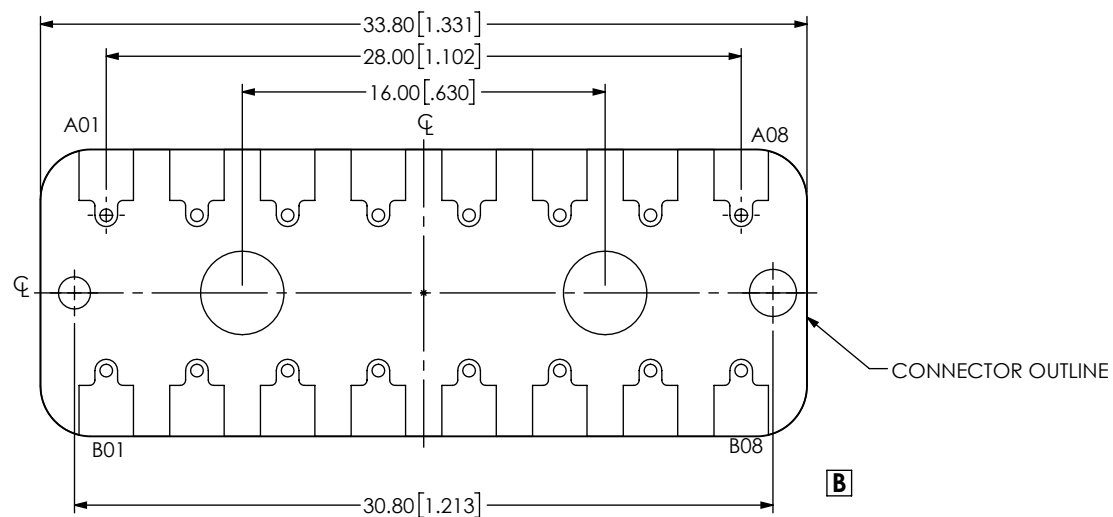
FIG 5 BE40A-M-XXXX-X-2-08-XXXX LAYOUT (DIFFERENT AS SHOWN, OTHERWISE SAME AS FIG 1)
