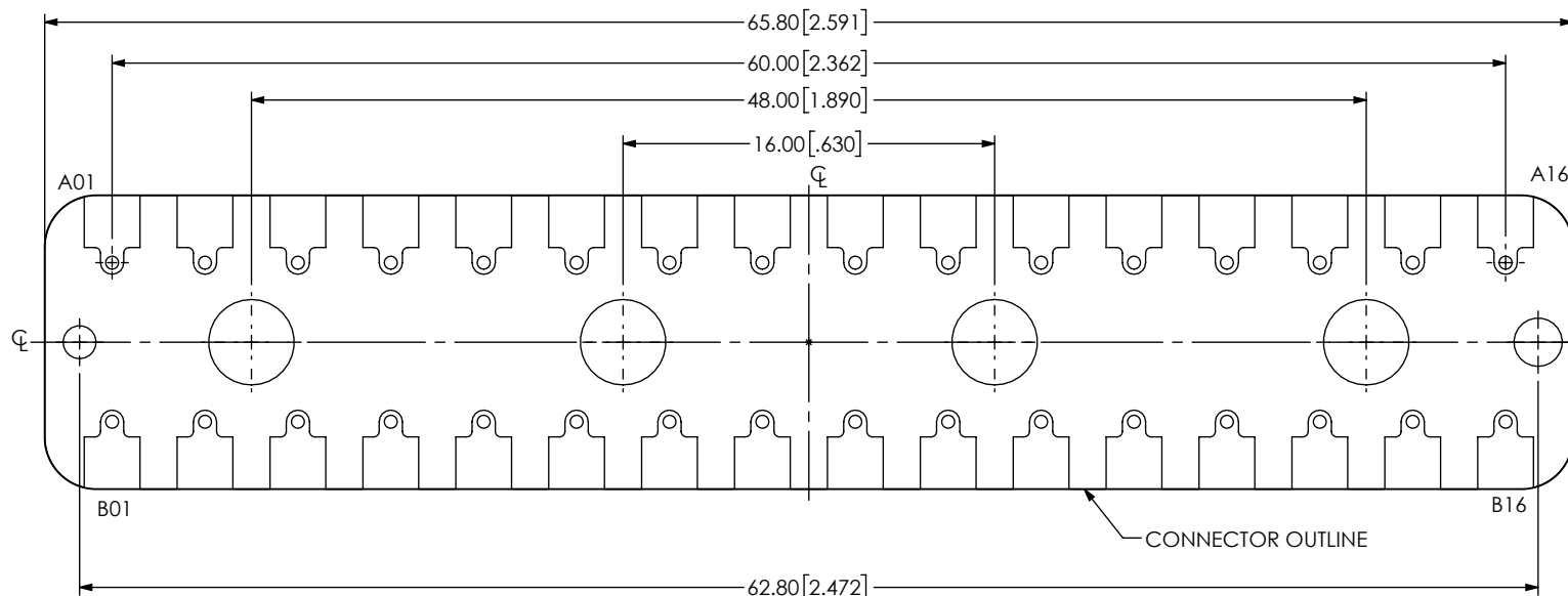
FIG 2 BE40A-M-XXXX-X-2-16-XXXX LAYOUT (DIFFERENT AS SHOWN, OTHERWISE SAME AS FIG 1)
