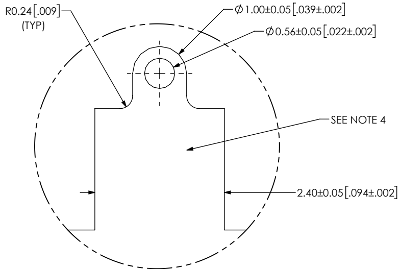
FIG 1 BE40A-M-XXXX-X-2-12-XXXX LAYOUT
