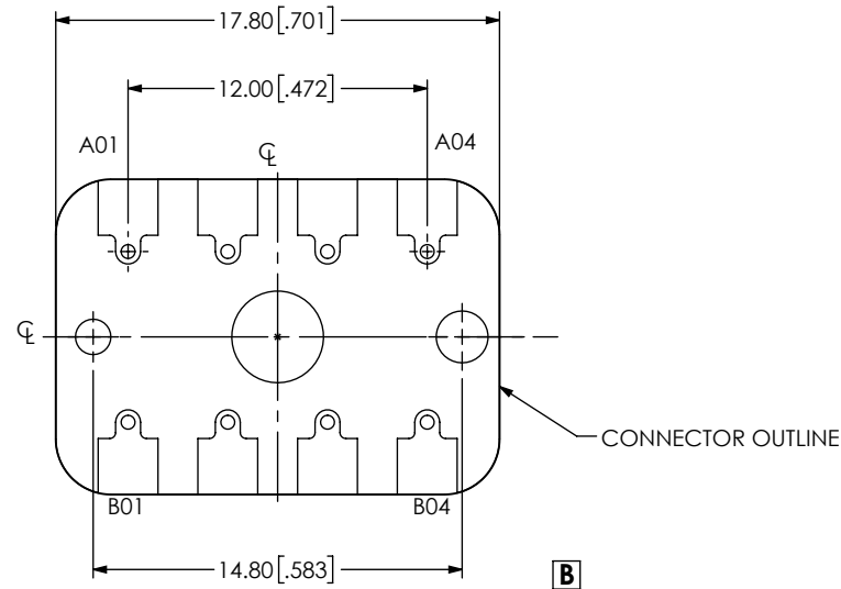
FIG 7 BE40A-M-XXXX-X-2-04-XXXX LAYOUT (DIFFERENT AS SHOWN, OTHERWISE SAME AS FIG 1)
