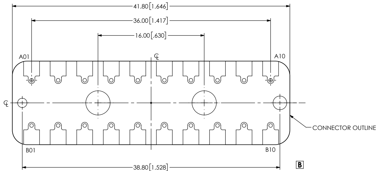
FIG 4 BE40A-M-XXXX-X-2-10-XXXX LAYOUT (DIFFERENT AS SHOWN, OTHERWISE SAME AS FIG 1)
