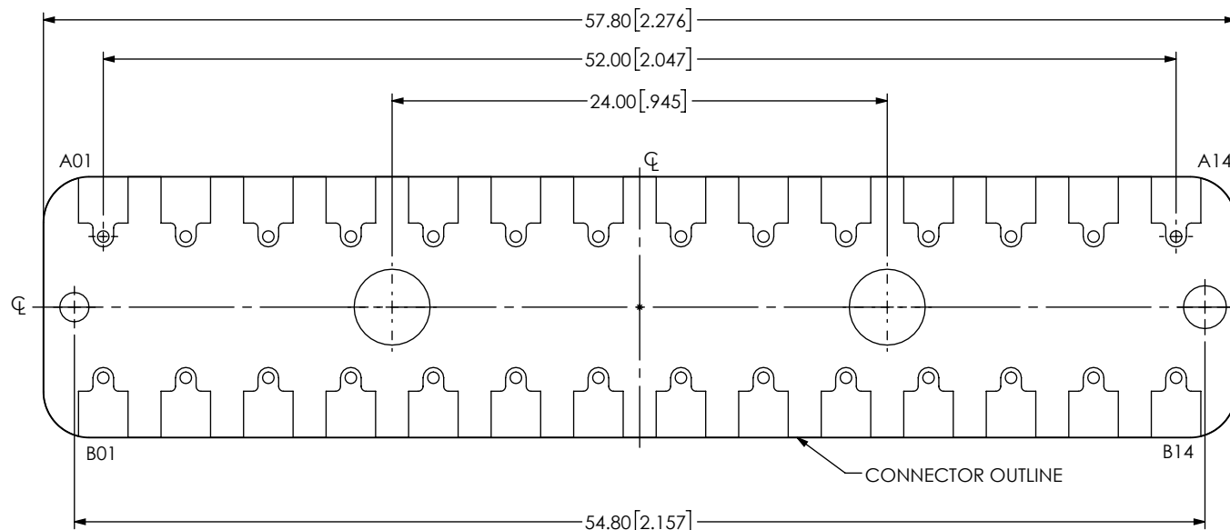
FIG 3 BE40A-M-XXXX-X-2-14-XXXX LAYOUT (DIFFERENT AS SHOWN, OTHERWISE SAME AS FIG 1)
