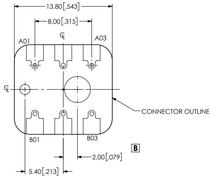
FIG 8 BE40A-M-XXXX-X-2-03-XXXX LAYOUT (DIFFERENT AS SHOWN, OTHERWISE SAME AS FIG 1)
