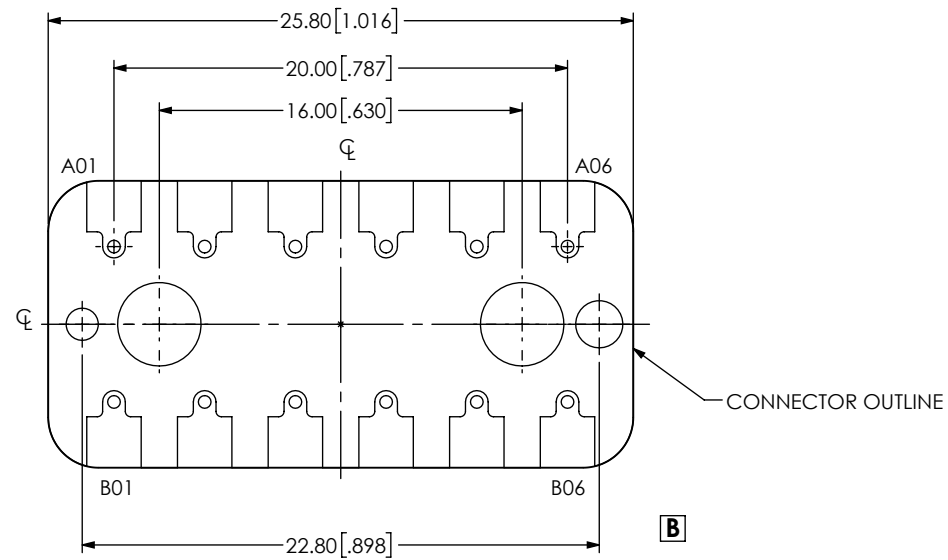
FIG 6 BE40A-M-XXXX-X-2-06-XXXX LAYOUT (DIFFERENT AS SHOWN, OTHERWISE SAME AS FIG 1)
