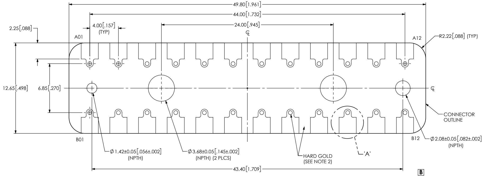
FIG 1 BE40A-M-XXXX-X-2-12-XXXX LAYOUT
