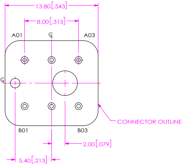
FIG 8 BE40A-S-XXXX-X-2-03-XXXX LAYOUT (DIFFERENT AS SHOWN, OTHERWISE SAME AS FIG 1)
