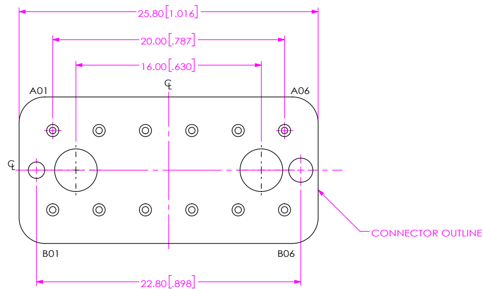
FIG 6 BE40A-S-XXXX-X-2-06-XXXX LAYOUT (DIFFERENT AS SHOWN, OTHERWISE SAME AS FIG 1)
