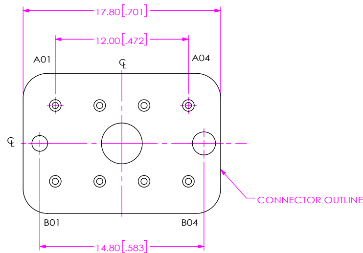
FIG 7 BE40A-S-XXXX-X-2-04-XXXX LAYOUT (DIFFERENT AS SHOWN, OTHERWISE SAME AS FIG 1)
