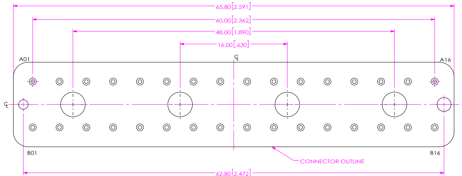
FIG 2 BE40A-S-XXXX-X-2-16-XXXX LAYOUT (DIFFERENT AS SHOWN, OTHERWISE SAME AS FIG 1)
