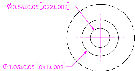
DETAIL 'A' SCALE 16:1 (TYPICAL ON ALL POSITIONS)
