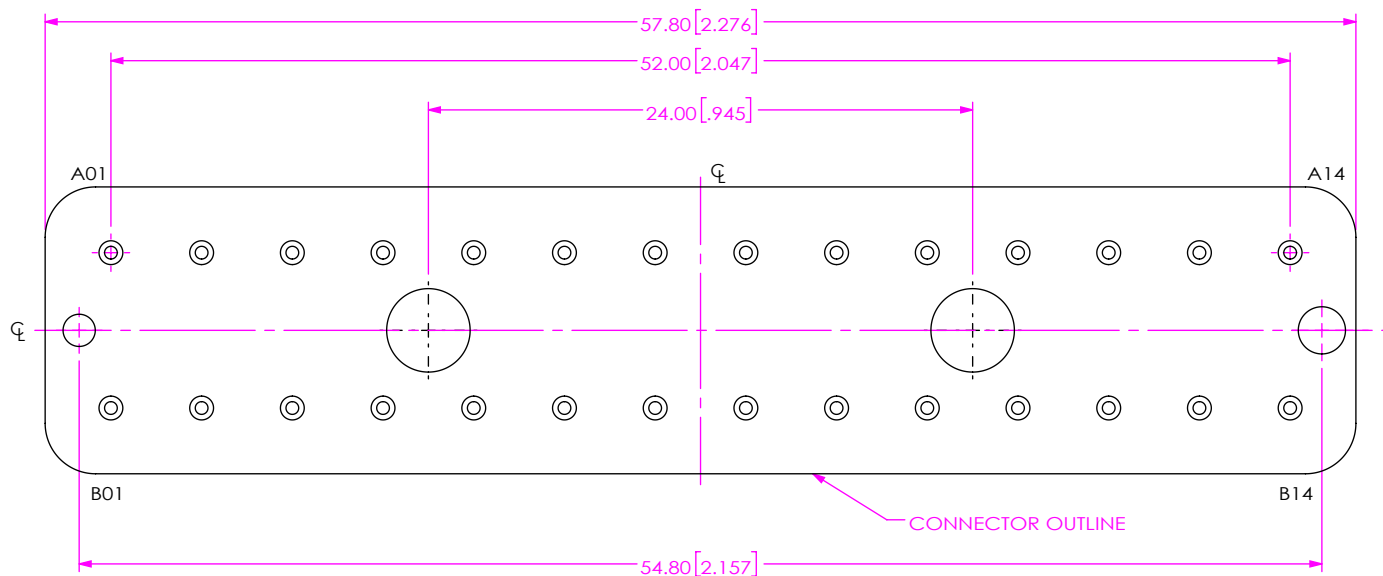
FIG 3 BE40A-S-XXXX-X-2-14-XXXX LAYOUT (DIFFERENT AS SHOWN, OTHERWISE SAME AS FIG 1)
