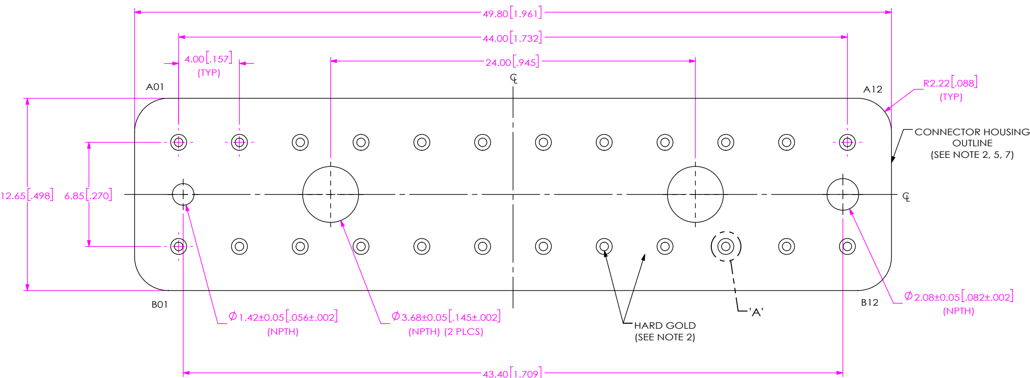
FIG 1 BE40A-S-XXXX-X-2-12-XXXX LAYOUT
