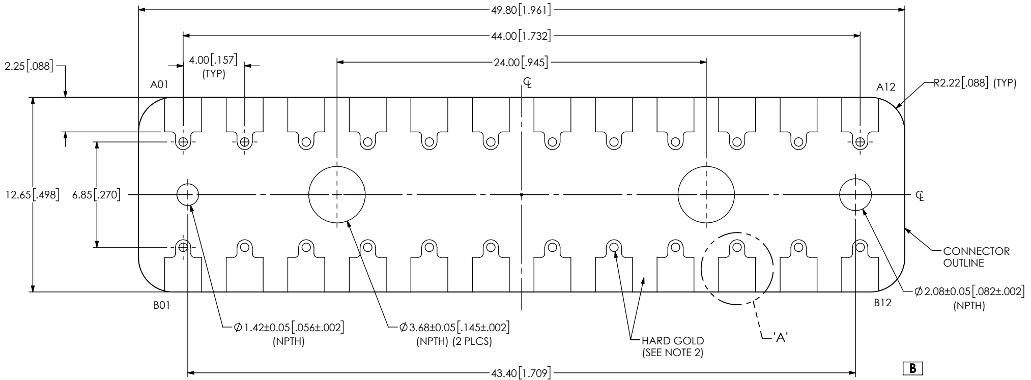
FIG 1 BE40B-J-M-2-12 LAYOUT
