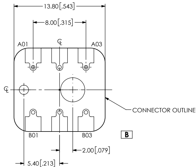
FIG 8 BE40B-J-M-2-03 LAYOUT (DIFFERENT AS SHOWN, OTHERWISE SAME AS FIG 1)
