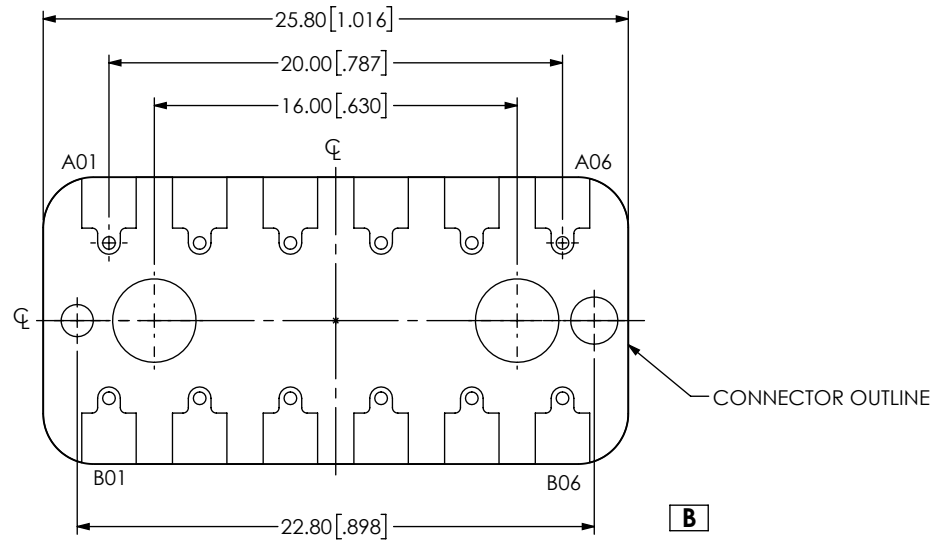
FIG 6 BE40B-J-M-2-06 LAYOUT (DIFFERENT AS SHOWN, OTHERWISE SAME AS FIG 1)
