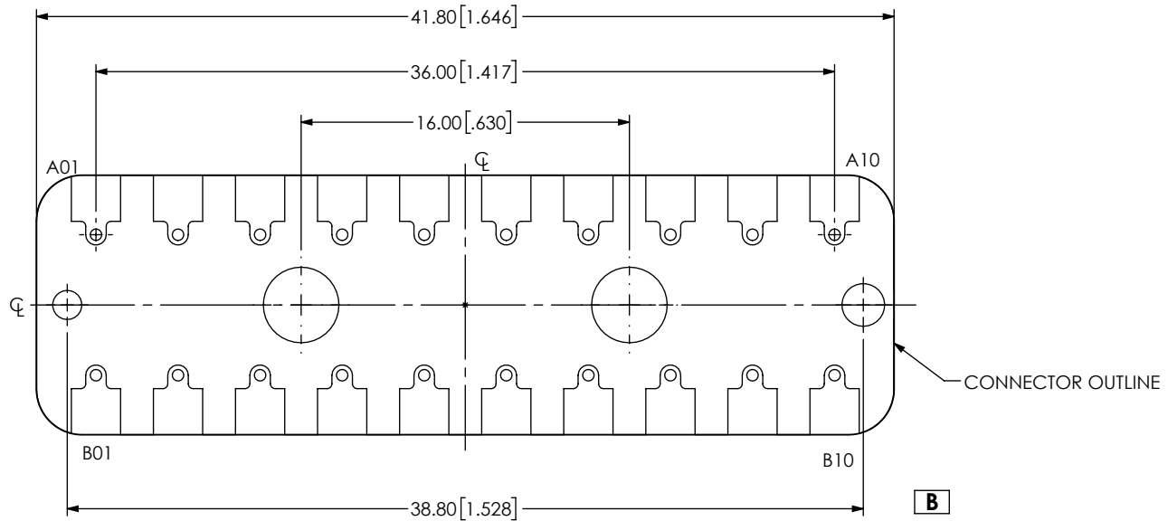
FIG 4 BE40B-J-M-2-10 LAYOUT (DIFFERENT AS SHOWN, OTHERWISE SAME AS FIG 1)
