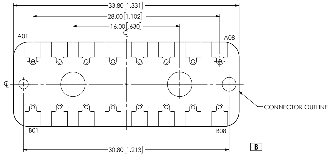
FIG 5 BE40B-J-M-2-08 LAYOUT (DIFFERENT AS SHOWN, OTHERWISE SAME AS FIG 1)
