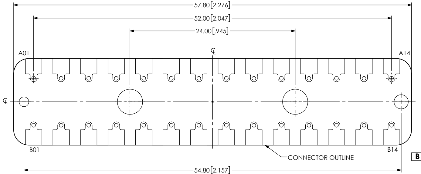
FIG 3 BE40B-J-M-2-14 LAYOUT (DIFFERENT AS SHOWN, OTHERWISE SAME AS FIG 1)
