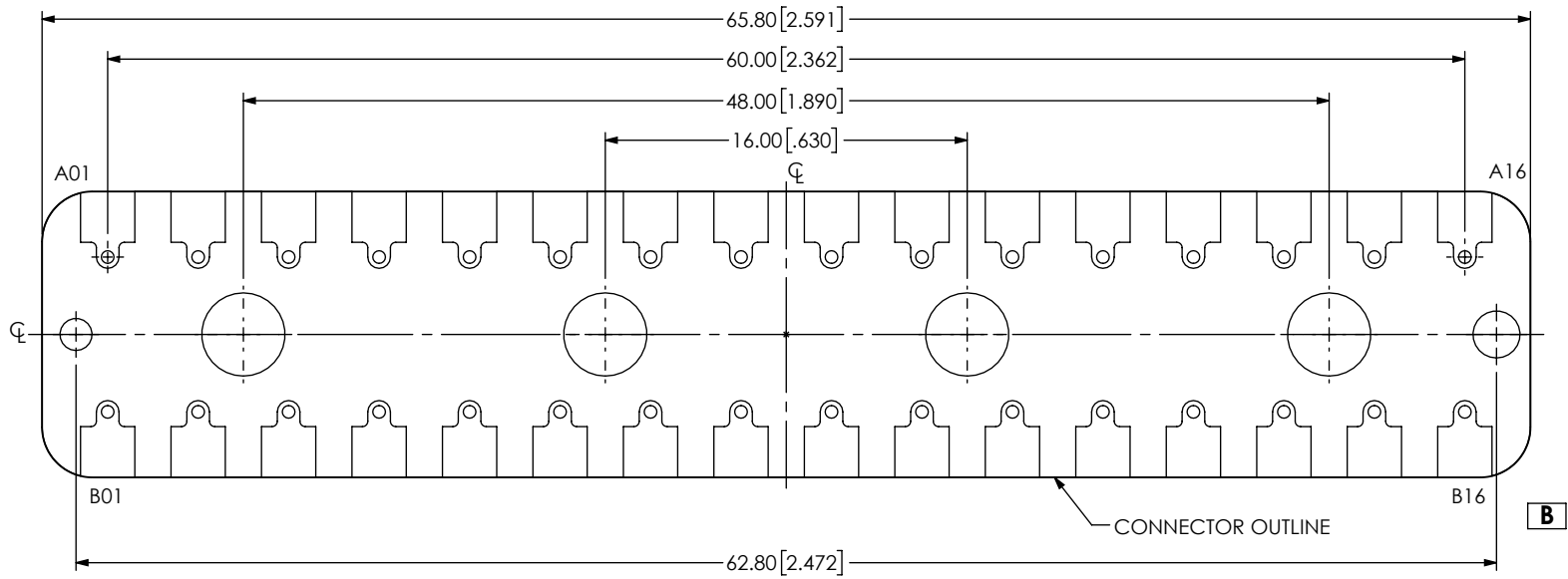
FIG 2 BE40B-J-M-2-16 LAYOUT (DIFFERENT AS SHOWN, OTHERWISE SAME AS FIG 1)
