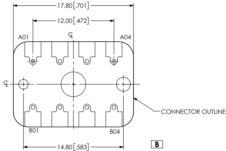
FIG 7 BE40B-J-M-2-04 LAYOUT (DIFFERENT AS SHOWN, OTHERWISE SAME AS FIG 1)
