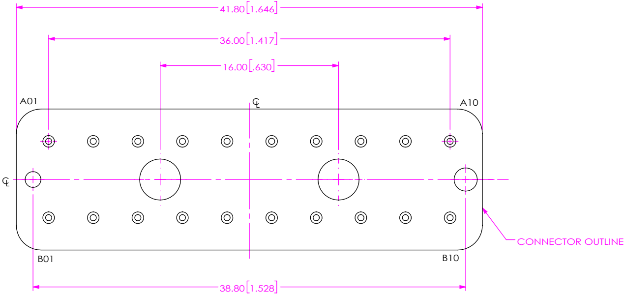
FIG 4 BE40B-J-S-2-10 LAYOUT (DIFFERENT AS SHOWN, OTHERWISE SAME AS FIG 1)
