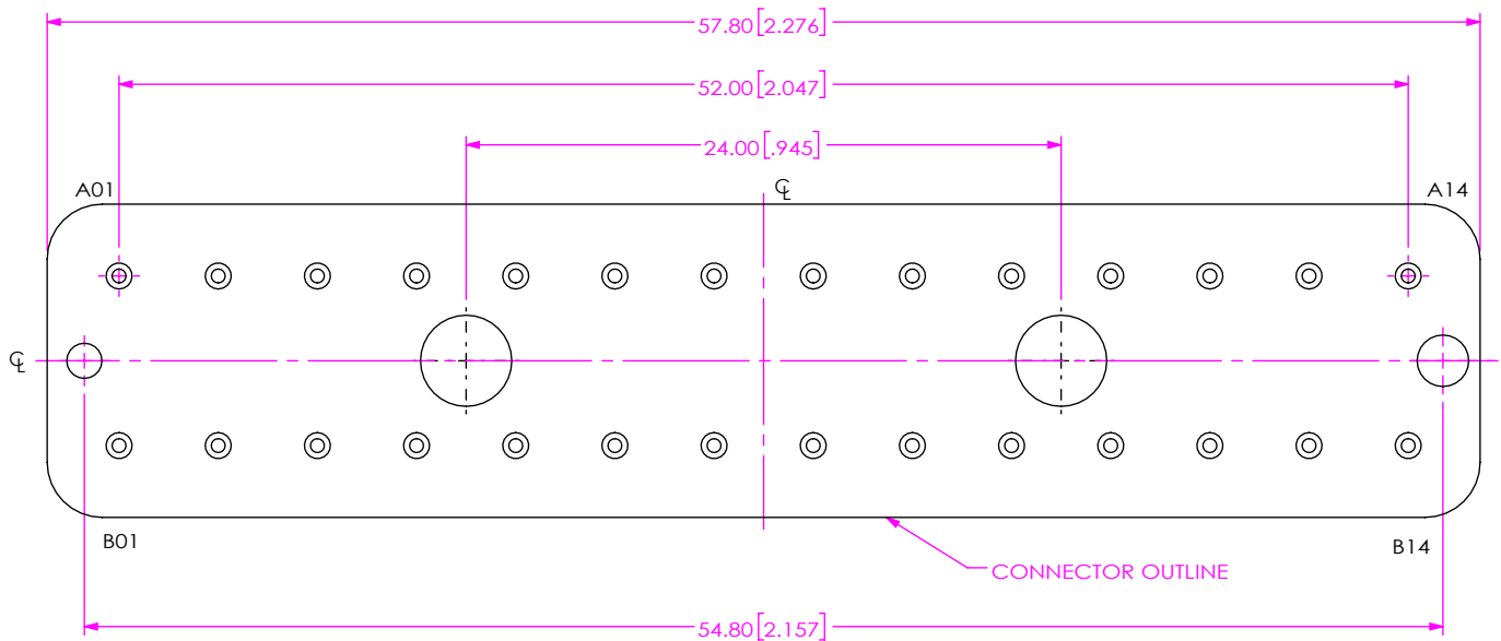
FIG 3 BE40B-J-S-2-14 LAYOUT (DIFFERENT AS SHOWN, OTHERWISE SAME AS FIG 1)
