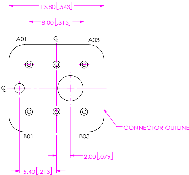
FIG 8 BE40B-J-S-2-03 LAYOUT (DIFFERENT AS SHOWN, OTHERWISE SAME AS FIG 1)
