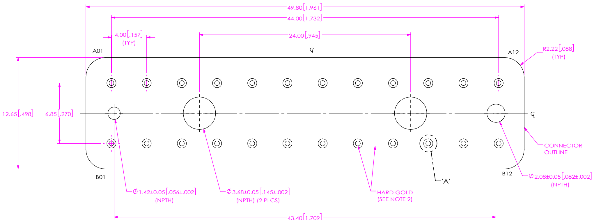
FIG 1 BE40B-J-S-2-12 LAYOUT
