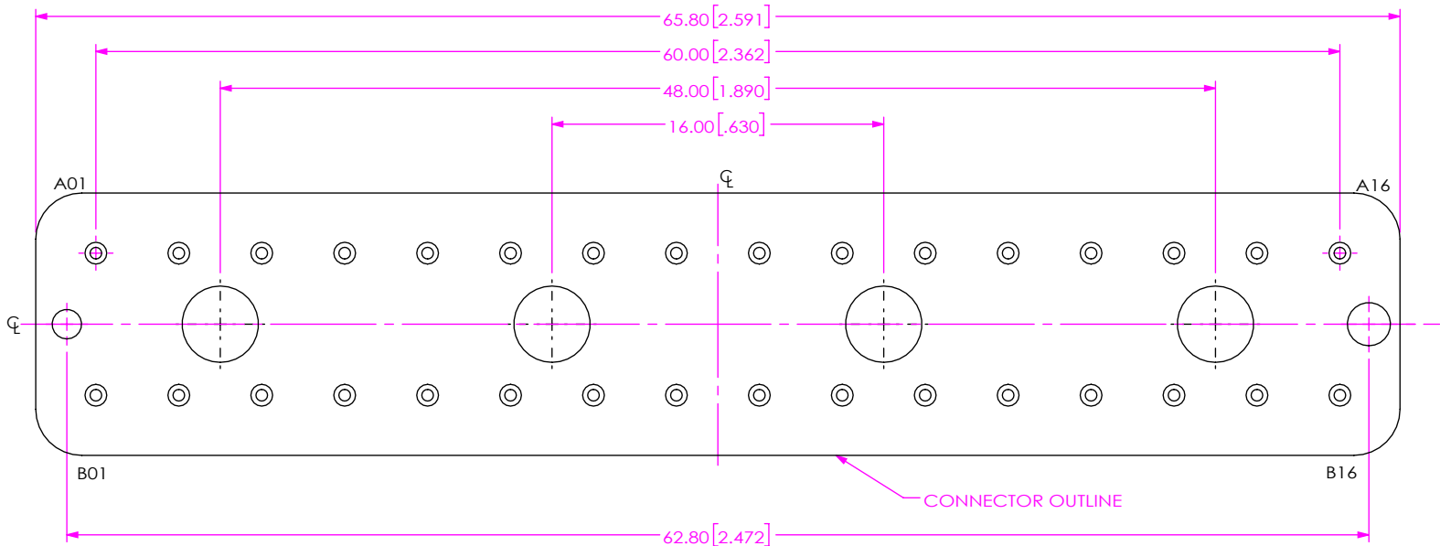
FIG 2 BE40B-J-S-2-16 LAYOUT (DIFFERENT AS SHOWN, OTHERWISE SAME AS FIG 1)
