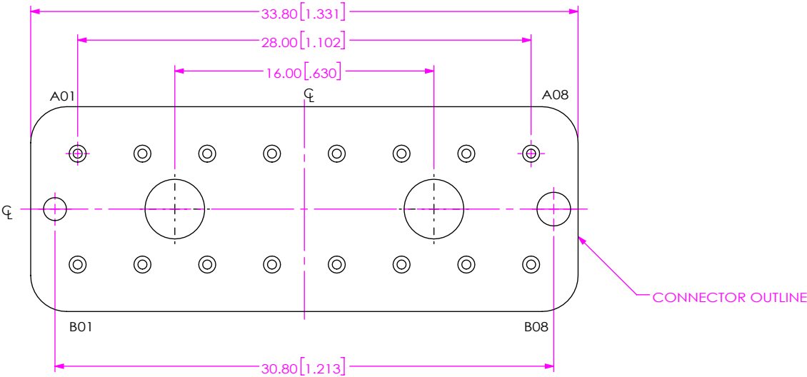
FIG 5 BE40B-J-S-2-08 LAYOUT (DIFFERENT AS SHOWN, OTHERWISE SAME AS FIG 1)
