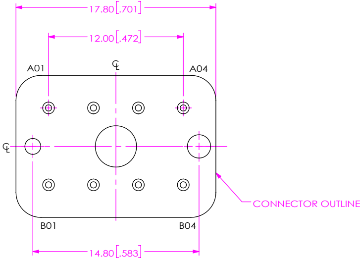
FIG 7 BE40B-J-S-2-04 LAYOUT (DIFFERENT AS SHOWN, OTHERWISE SAME AS FIG 1)
