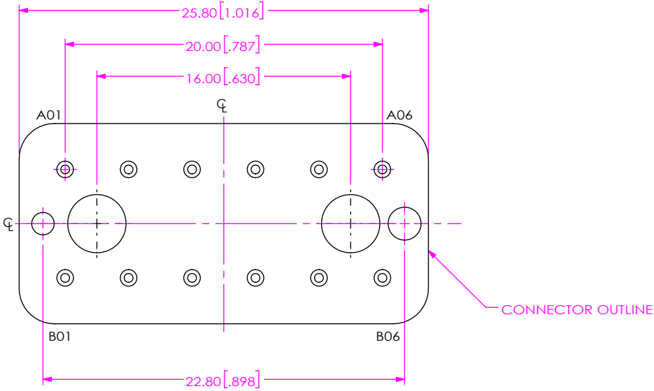
FIG 6 BE40B-J-S-2-06 LAYOUT (DIFFERENT AS SHOWN, OTHERWISE SAME AS FIG 1)
