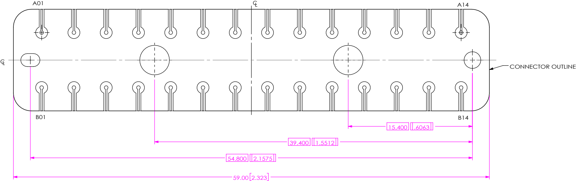
FIG 3 BE70A-M-XXXX-X-2-14-XXXX LAYOUT (DIFFERENT AS SHOWN, OTHERWISE SAME AS FIG 1)
