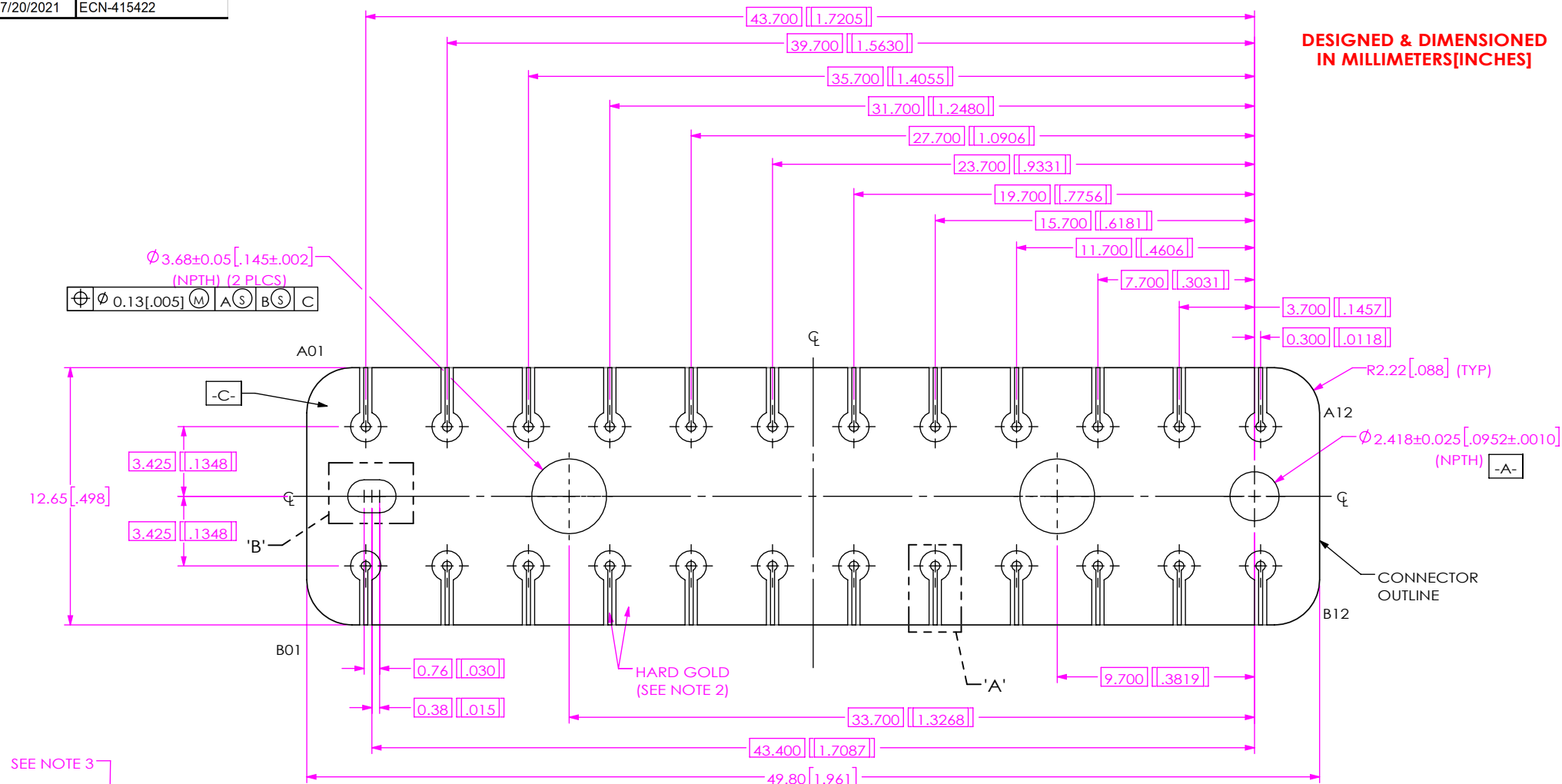
FIG 1 BE70A-M-XXXX-X-2-12-XXXX LAYOUT
