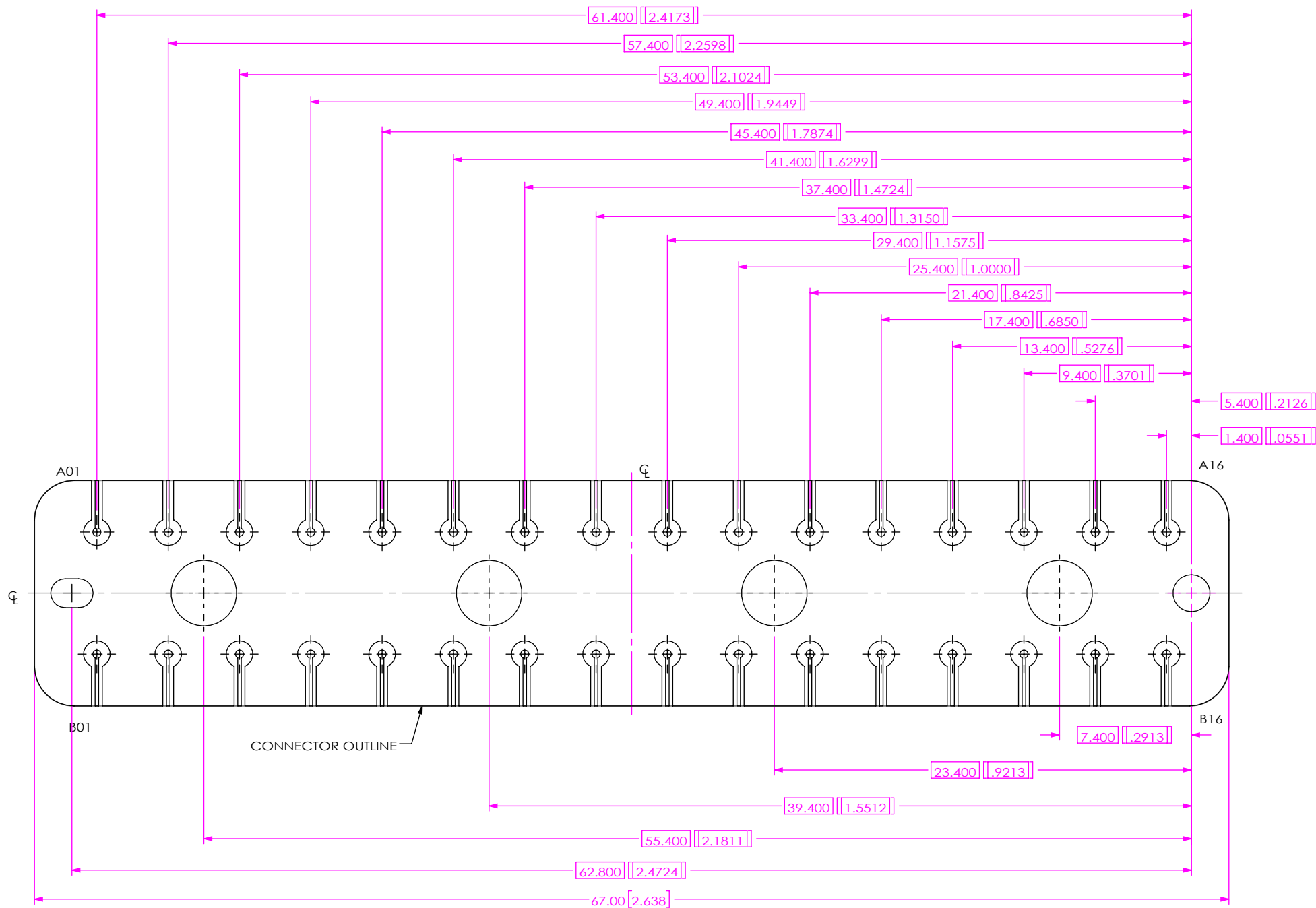
FIG 2 BE70A-M-XXXX-X-2-16-XXXX LAYOUT (DIFFERENT AS SHOWN, OTHERWISE SAME AS FIG 1)
