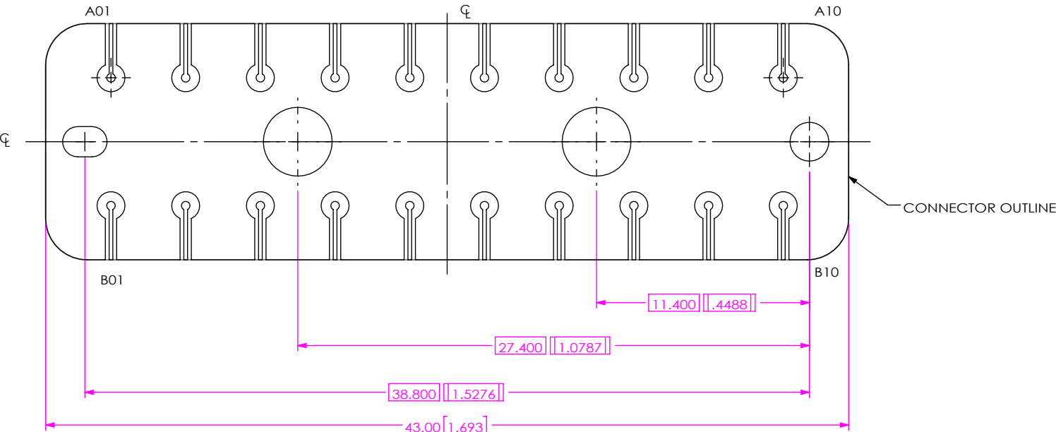
FIG 4 BE70A-M-XXXX-X-2-10-XXXX LAYOUT (DIFFERENT AS SHOWN, OTHERWISE SAME AS FIG 1)
