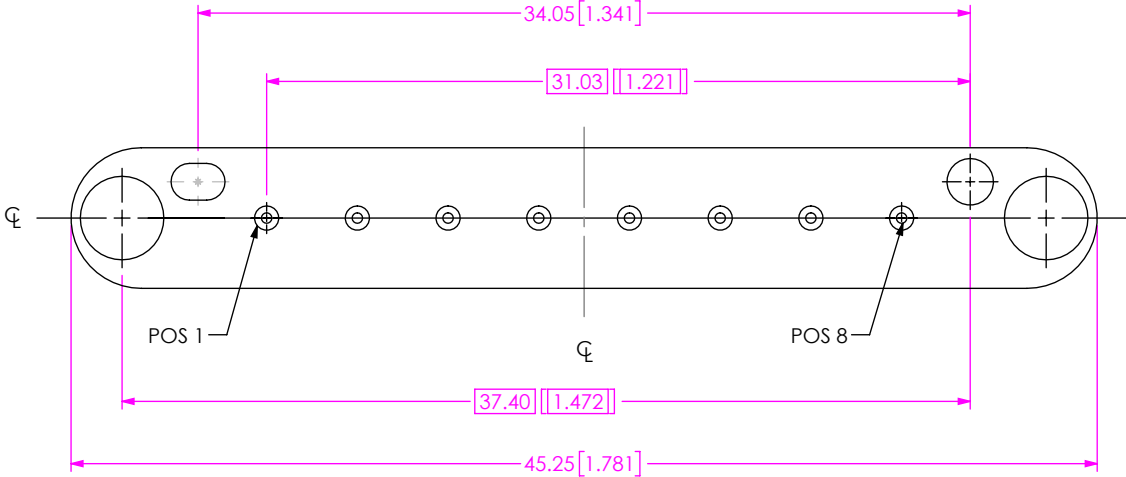
FIG 2 BE70A-S-XXXX-X-1-08-XXXX LAYOUT (DIFFERENT AS SHOWN, OTHERWISE SAME AS FIG 1)
