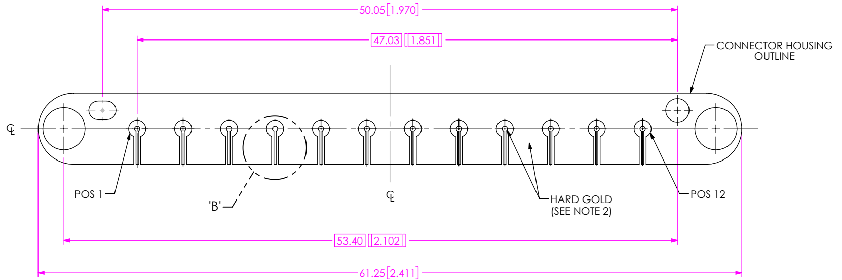
FIG 5 BE70A-M-XXXX-X-T2-XXXX LAYOUT (DIFFERENT AS SHOWN, OTHERWISE SAME AS FIG 1)
