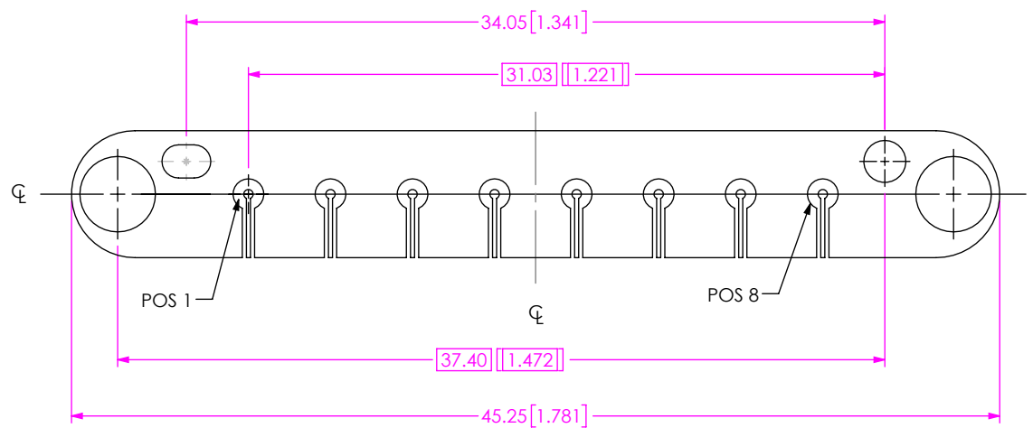
FIG 6 BE70A-M-XXXX-X-1-08-XXXX LAYOUT (DIFFERENT AS SHOWN, OTHERWISE SAME AS FIG 5)
