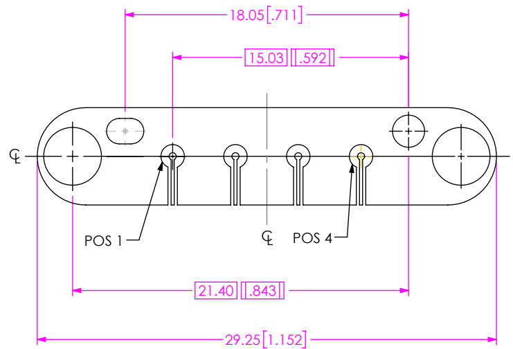
FIG 7 BE70A-M-XXXX-X-1-04-XXXX LAYOUT (DIFFERENT AS SHOWN, OTHERWISE SAME AS FIG 5)
