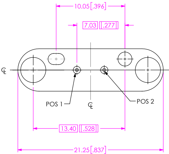
FIG 4 BE70A-S-XXXX-X-1-02-XXXX LAYOUT (DIFFERENT AS SHOWN, OTHERWISE SAME AS FIG 1)
