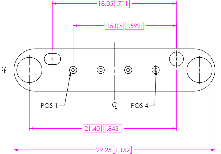
FIG 3 BE70A-S-XXXX-X-1-04-XXXX LAYOUT (DIFFERENT AS SHOWN, OTHERWISE SAME AS FIG 1)
