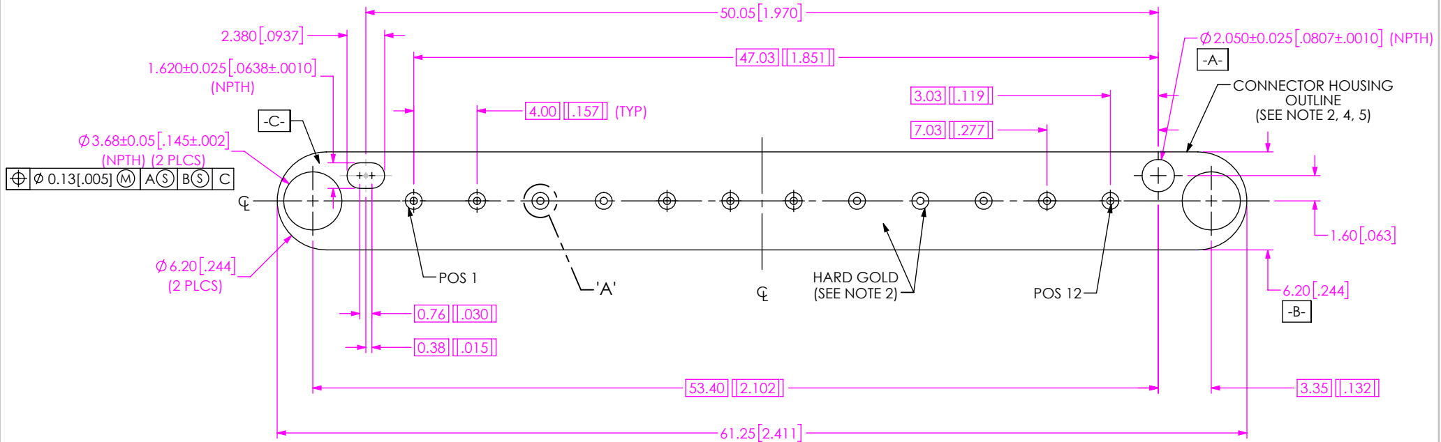
FIG 1 BE70A-S-XXXX-X-1-12-XXXX LAYOUT
