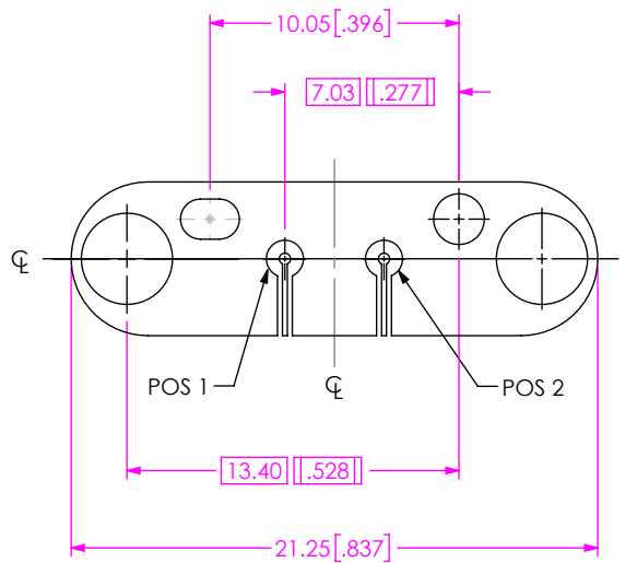
FIG 8 BE70A-M-XXXX-X-1-02-XXXX LAYOUT (DIFFERENT AS SHOWN, OTHERWISE SAME AS FIG 5)
