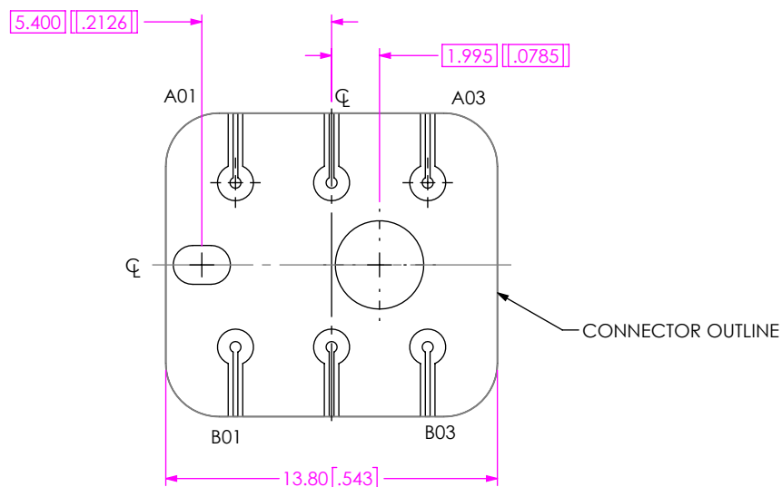
FIG 8 BE71A-M-XXXX-X-2-03-XXXX LAYOUT (DIFFERENT AS SHOWN, OTHERWISE SAME AS FIG 1)
