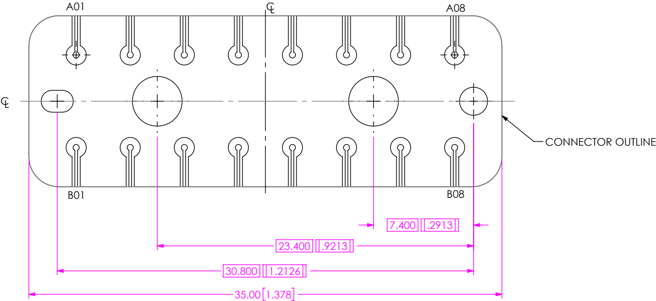
FIG 5 BE71A-M-XXXX-X-2-08-XXXX LAYOUT (DIFFERENT AS SHOWN, OTHERWISE SAME AS FIG 1)
