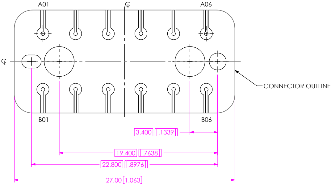
FIG 6 BE71A-M-XXXX-X-2-06-XXXX LAYOUT (DIFFERENT AS SHOWN, OTHERWISE SAME AS FIG 1)
