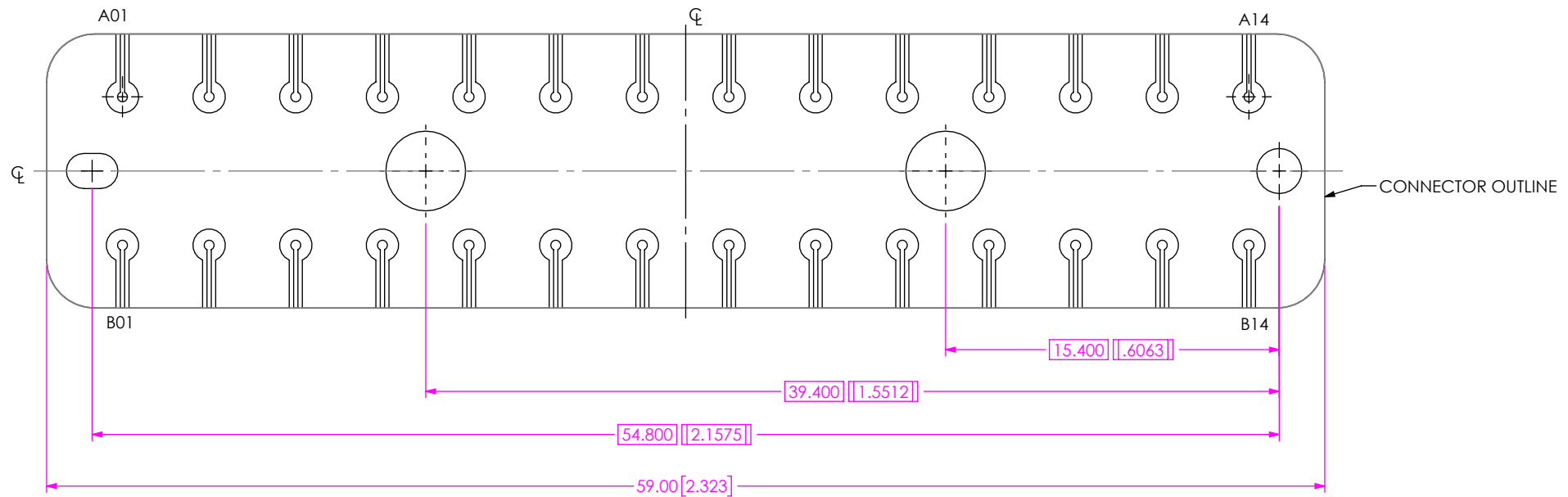
FIG 3 BE71A-M-XXXX-X-2-14-XXXX LAYOUT (DIFFERENT AS SHOWN, OTHERWISE SAME AS FIG 1)
