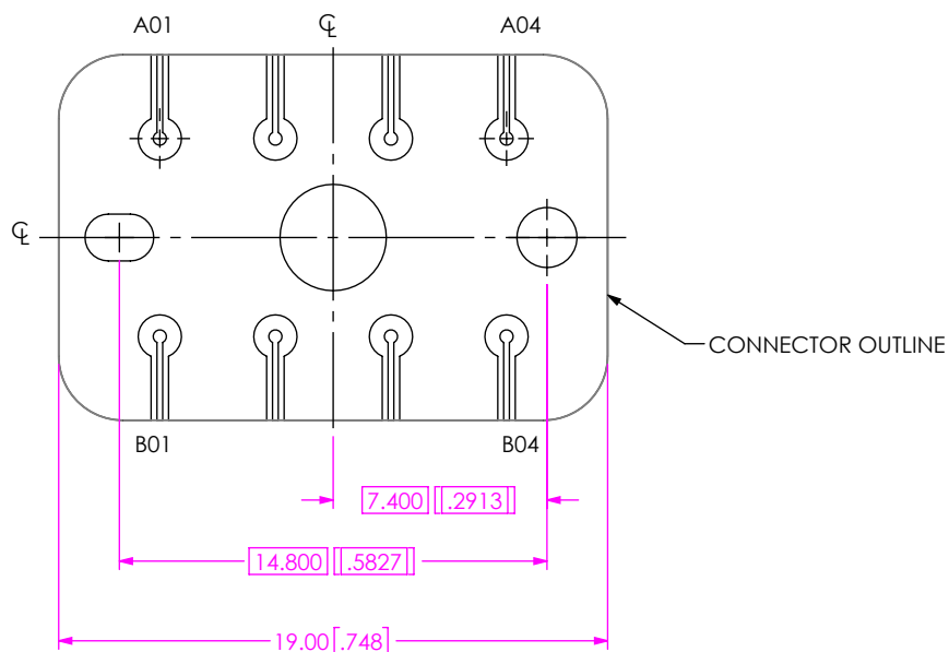
FIG 7 BE71A-M-XXXX-X-2-04-XXXX LAYOUT (DIFFERENT AS SHOWN, OTHERWISE SAME AS FIG 1)
