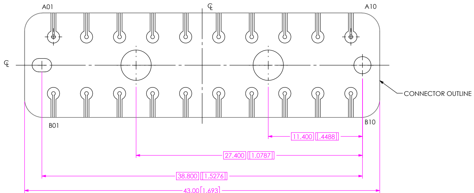
FIG 4 BE71A-M-XXXX-X-2-10-XXXX LAYOUT (DIFFERENT AS SHOWN, OTHERWISE SAME AS FIG 1)
