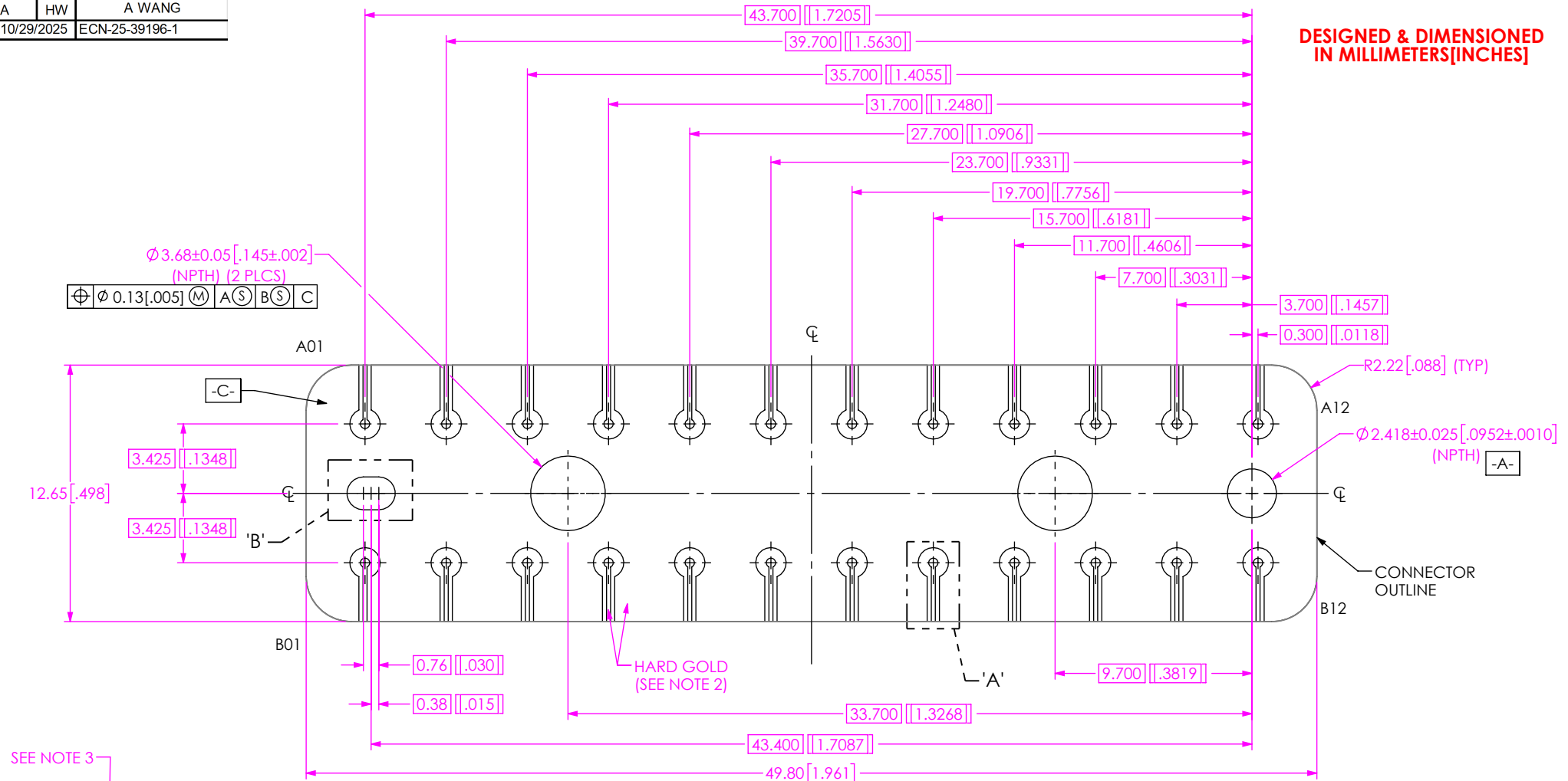
FIG 1 BE71A-M-XXXX-X-2-12-XXXX LAYOUT
