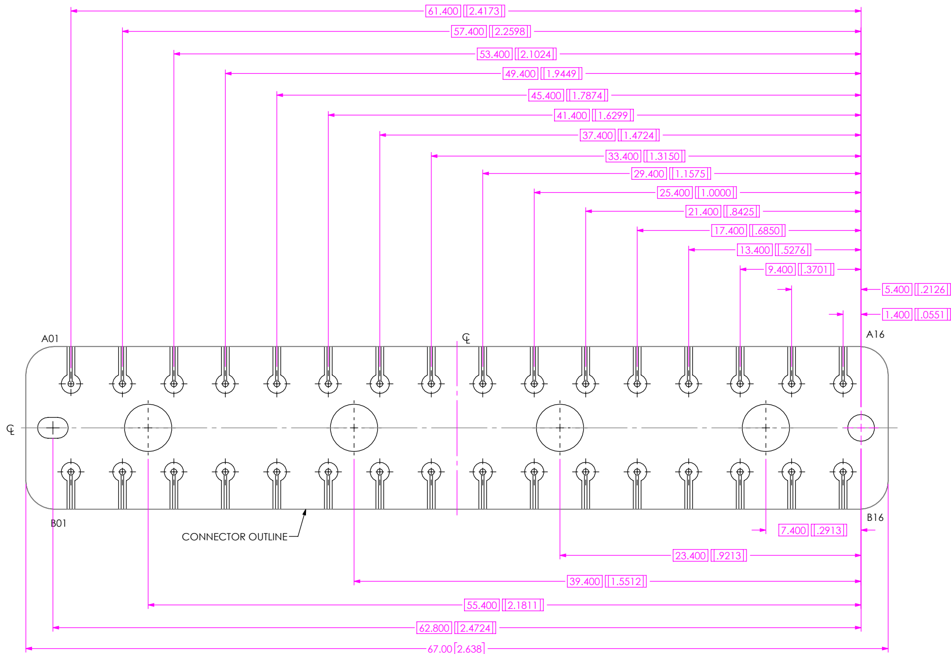
FIG 2 BE71A-M-XXXX-X-2-16-XXXX LAYOUT (DIFFERENT AS SHOWN, OTHERWISE SAME AS FIG 1)
