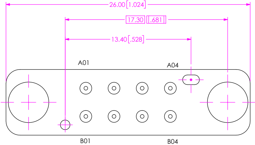
FIG 4 BE90A-S-XXXX-X-2-04-XXXX LAYOUT (DIFFERENT AS SHOWN, OTHERWISE SAME AS FIG 1)
