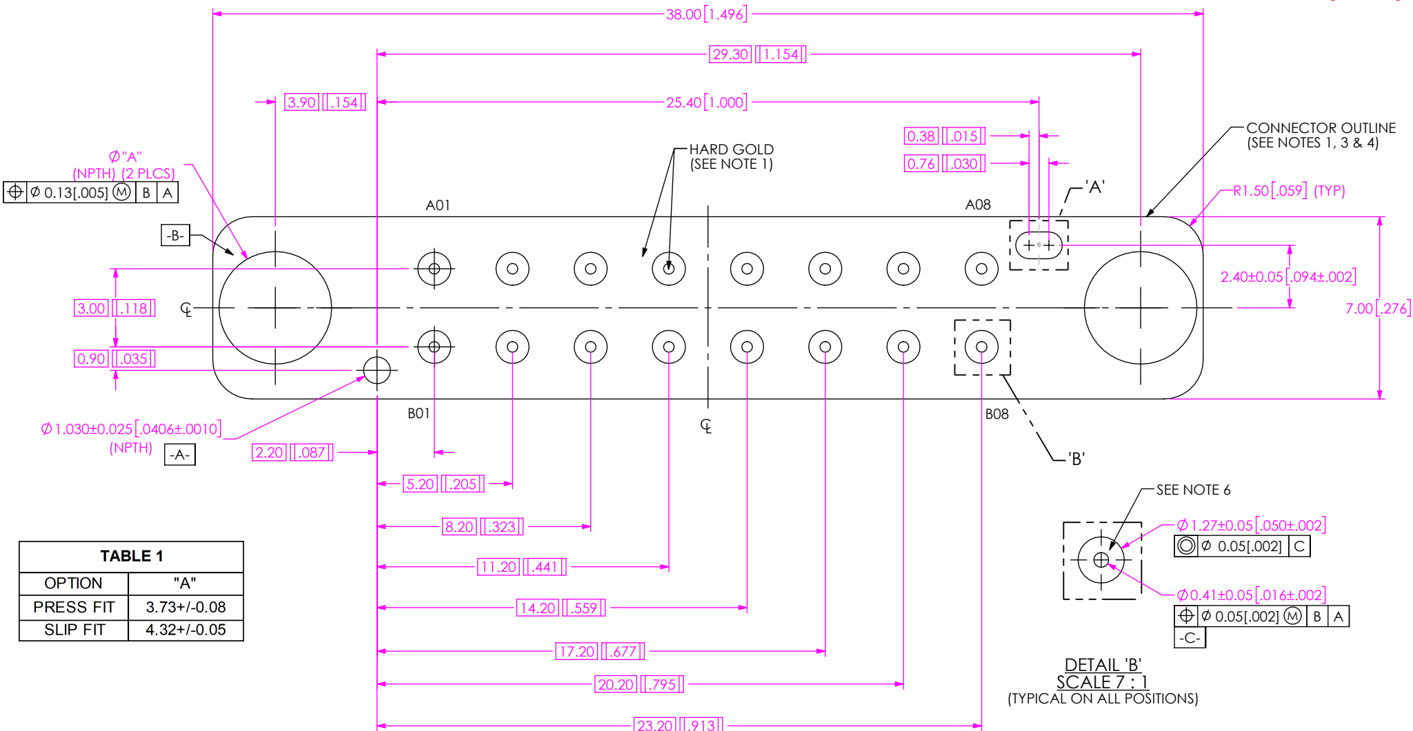
FIG 1 BE90A-S-XXXX-X-2-08-XXXX LAYOUT
