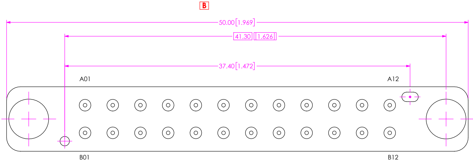
FIG 3 BE90A-S-XXXX-X-2-12-XXXX LAYOUT (DIFFERENT AS SHOWN, OTHERWISE SAME AS FIG 1)
