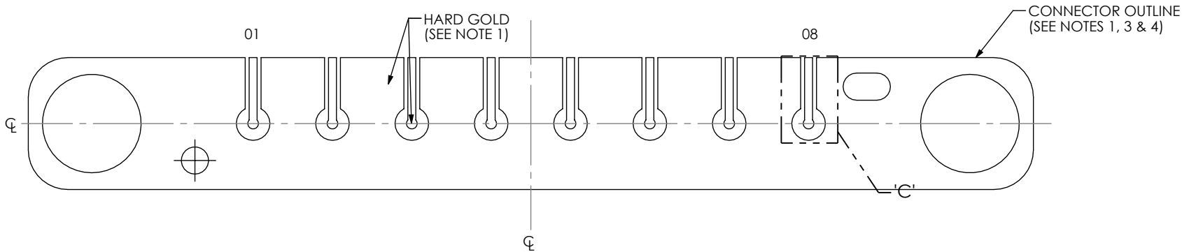
FIG 5 BE90A-M-XXXX-X-1-08-XXXX LAYOUT (DIFFERENT AS SHOWN, OTHERWISE SAME AS FIG 1)
