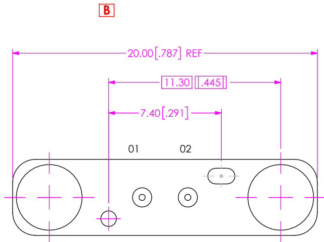
FIG 3 BE90A-S-XXXX-X-1-02-XXXX LAYOUT (DIFFERENT AS SHOWN, OTHERWISE SAME AS FIG 1)
