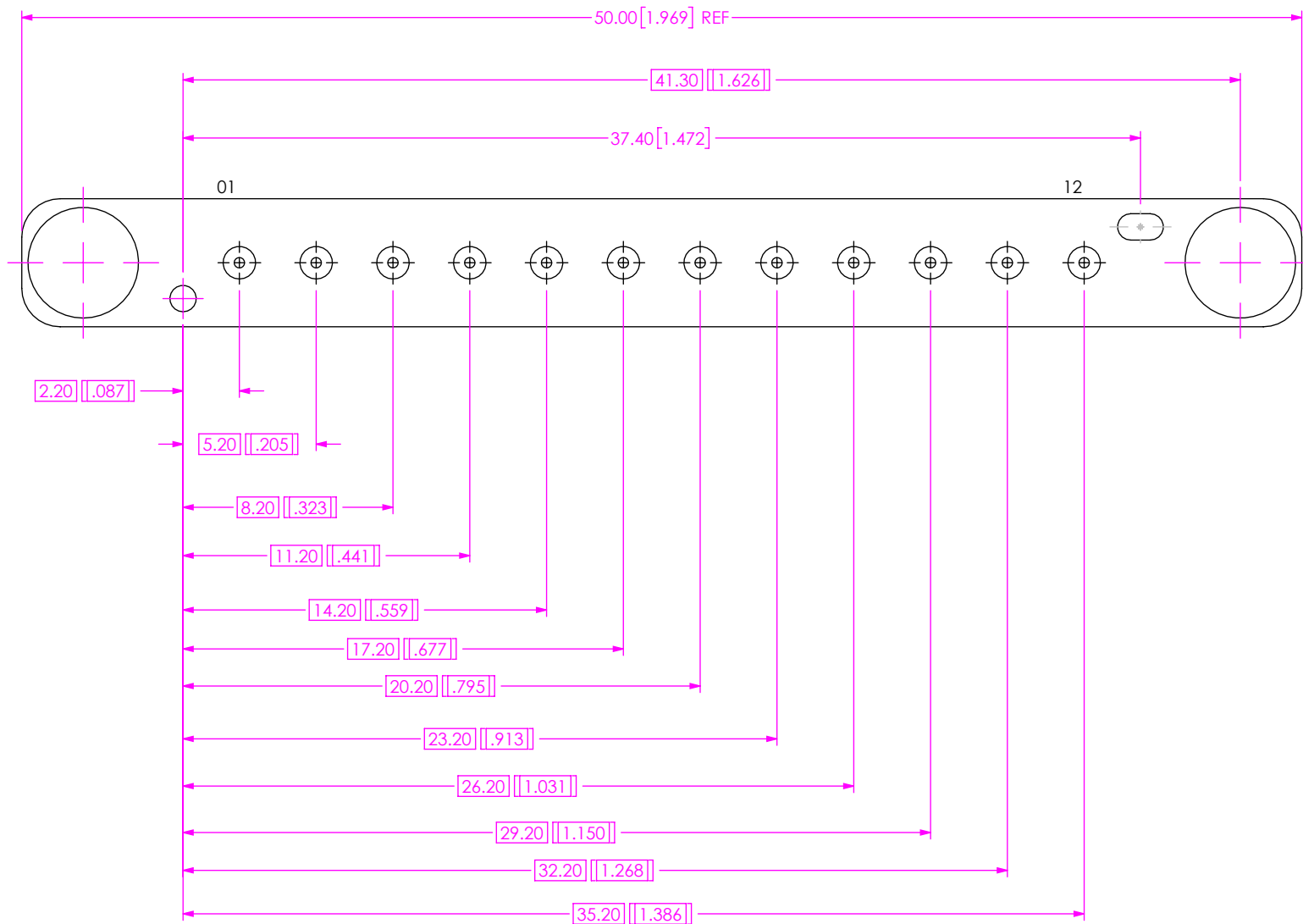
FIG 2 BE90A-S-XXXX-X-1-12-XXXX LAYOUT (DIFFERENT AS SHOWN, OTHERWISE SAME AS FIG 1)
