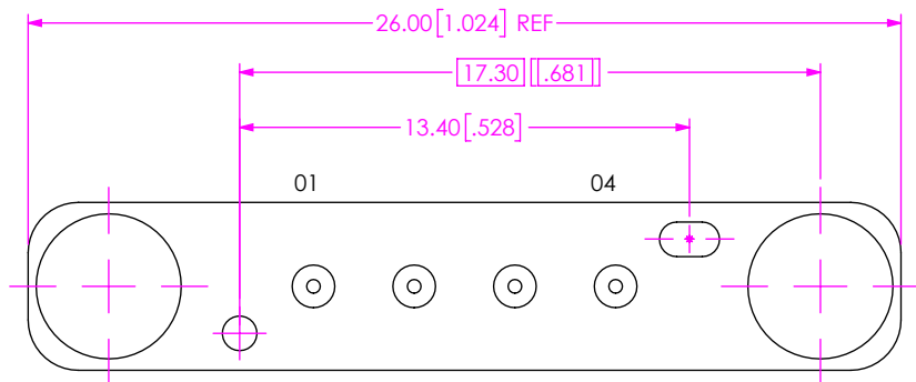
FIG 4 BE90A-S-XXXX-X-1-04-XXXX LAYOUT (DIFFERENT AS SHOWN, OTHERWISE SAME AS FIG 1)
