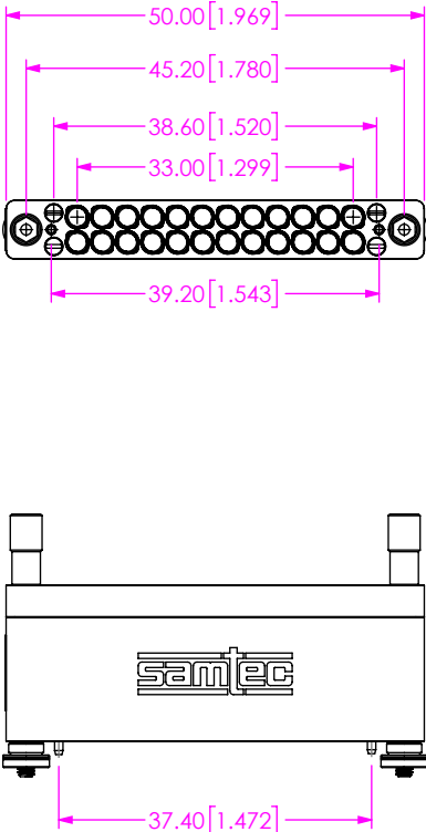
FIG 9 BE90A-S-XXXX-X-2-12-XXXX SHOWN (CABLE ASSEMBLIES NOT SHOWN FOR CLARITY)
