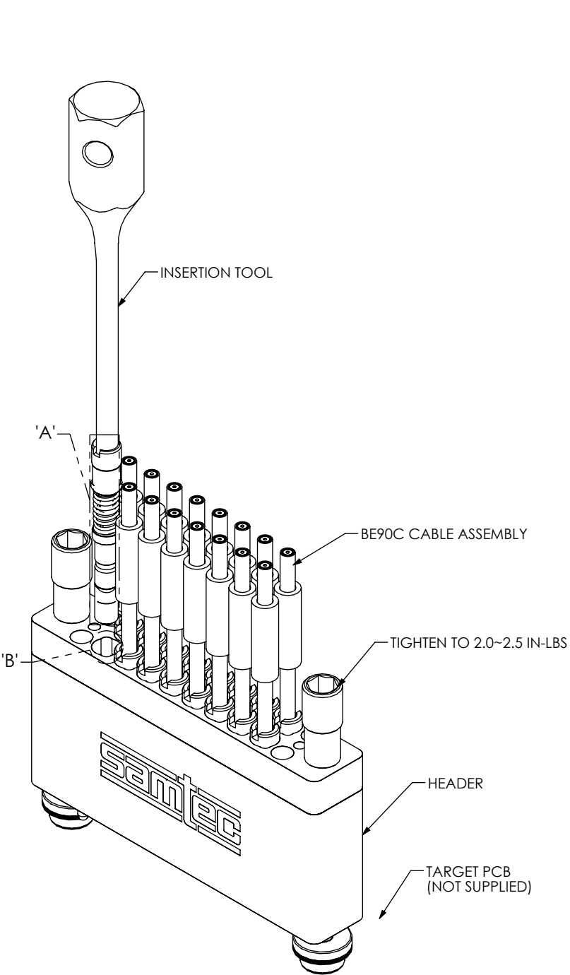
APPLICATION VIEW FOR CABLE ASSEMBLY
