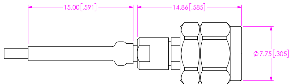
FIG 13 -24SP SHOWN (CABLE CUT FOR CLARITY ONLY)
