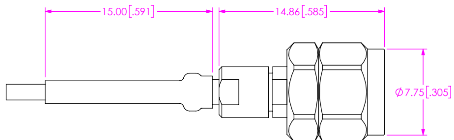
FIG 11 -18SP SHOWN (CABLE CUT FOR CLARITY ONLY)
