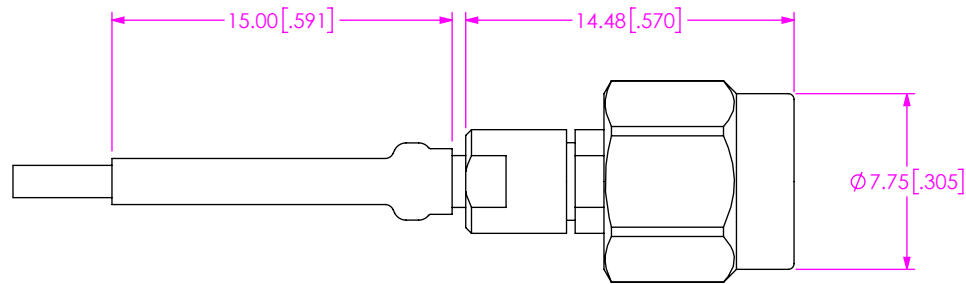
FIG 15 -92SP SHOWN (CABLE CUT FOR CLARITY ONLY)
