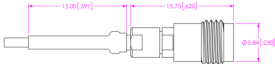
FIG 14 -24SJ SHOWN (CABLE CUT FOR CLARITY ONLY)
