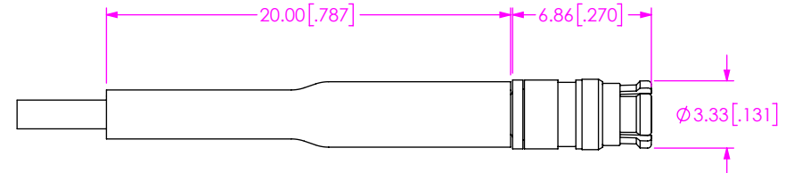
FIG 18 -00SJ SHOWN (CABLE CUT FOR CLARITY ONLY)
