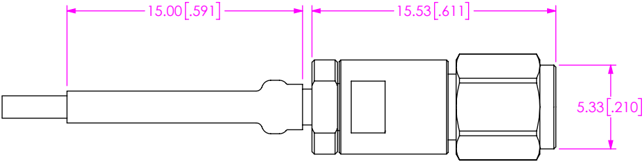
FIG 5 -10SP SHOWN (CABLE CUT FOR CLARITY ONLY)
