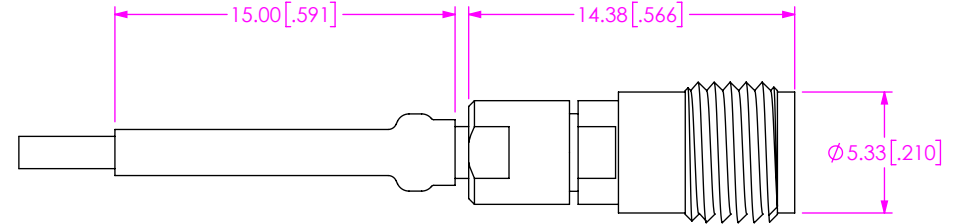
FIG 16 -92SJ SHOWN (CABLE CUT FOR CLARITY ONLY)
