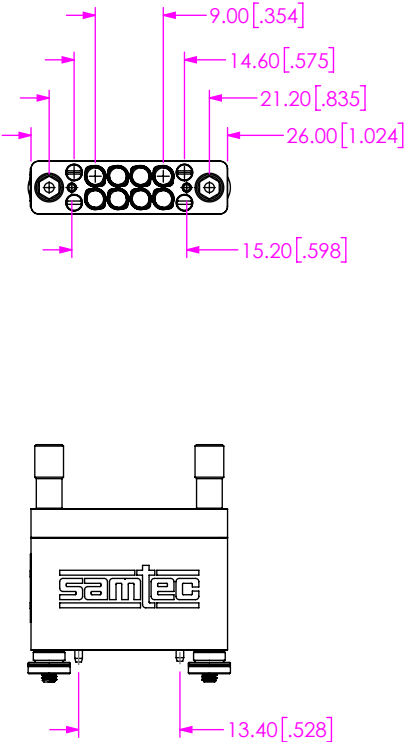
FIG 10 BE90A-S-XXXX-X-2-04-XXXX SHOWN (CABLE ASSEMBLIES NOT SHOWN FOR CLARITY)
