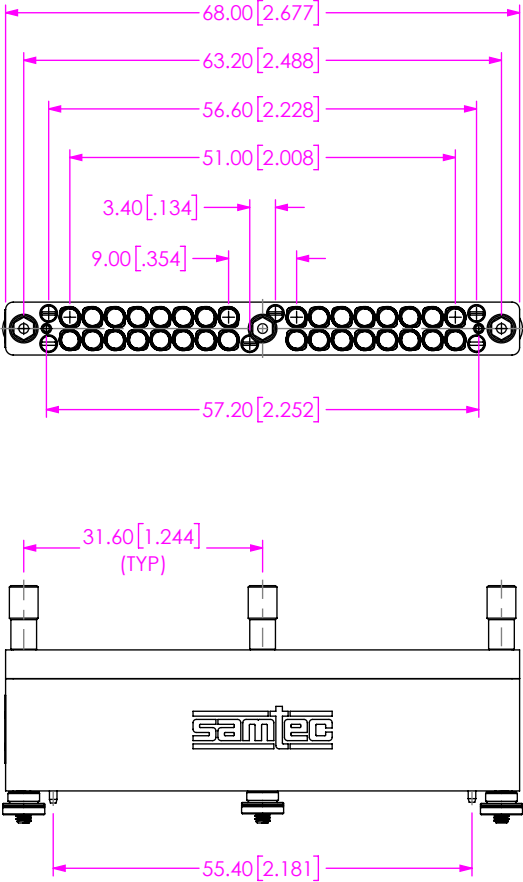
FIG 8 BE90A-S-XXXX-X-2-16-XXXX SHOWN (CABLE ASSEMBLIES NOT SHOWN FOR CLARITY)
