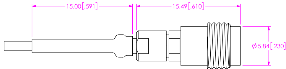
FIG 12 -18SJ SHOWN (CABLE CUT FOR CLARITY ONLY)
