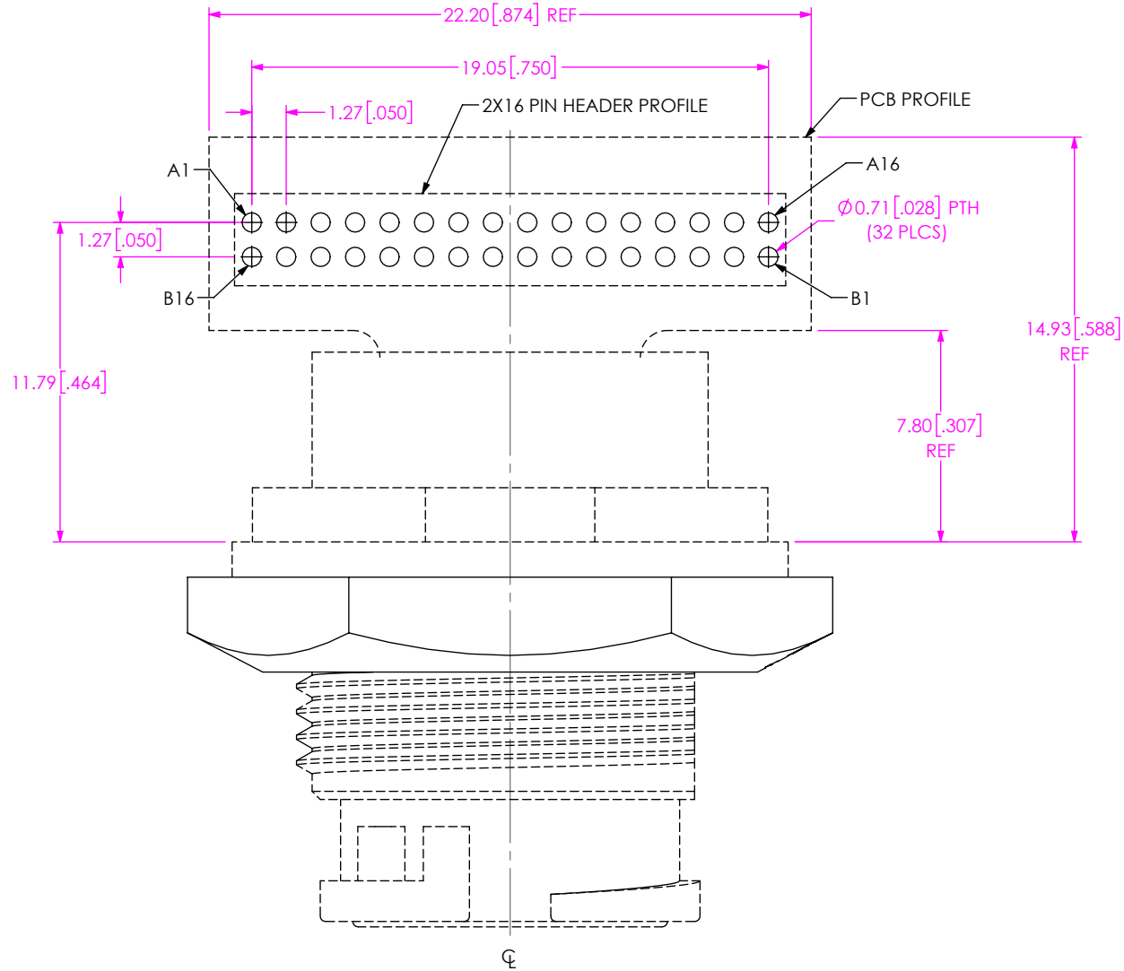
FIG 2 BRU-C-S-RA-P SHOWN ALL DIMENSIONS ARE SYMMETRIC ABOUT THE CENTERLINE. RECOMMENDED PCB THICKNESS: 1.6MM[.062"]
