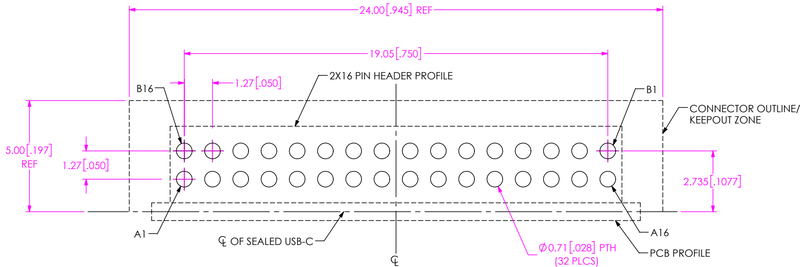
FIG 1 BRU-C-S-VT-P SHOWN ALL DIMENSIONS ARE SYMMETRIC ABOUT THE CENTERLINE. RECOMMENDED PCB THICKNESS: 2.4MM[.093"]
