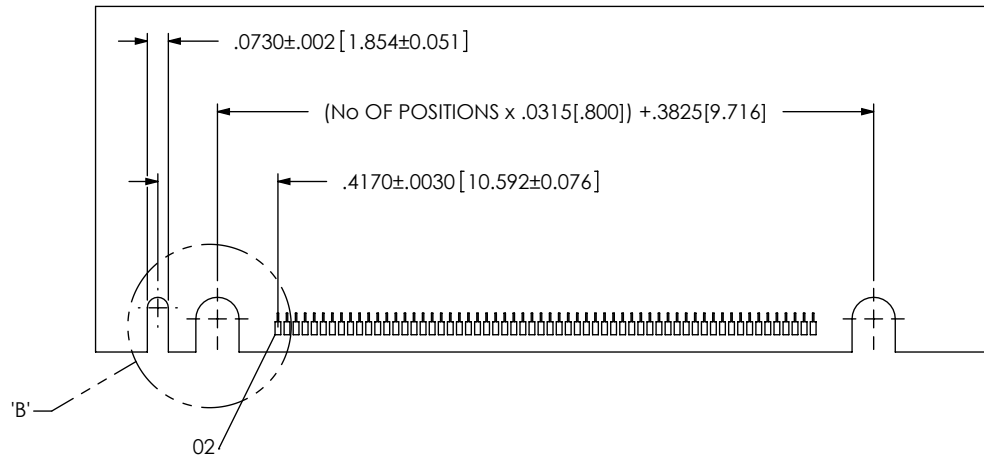
FIG 2: RECOMMENDED PCB LAYOUT FOR -GP DESIGNS [DIFFERENT AS SHOWN, OTHERWISE SAE AS FIG 1]
