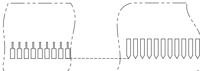
PCB DETAIL
