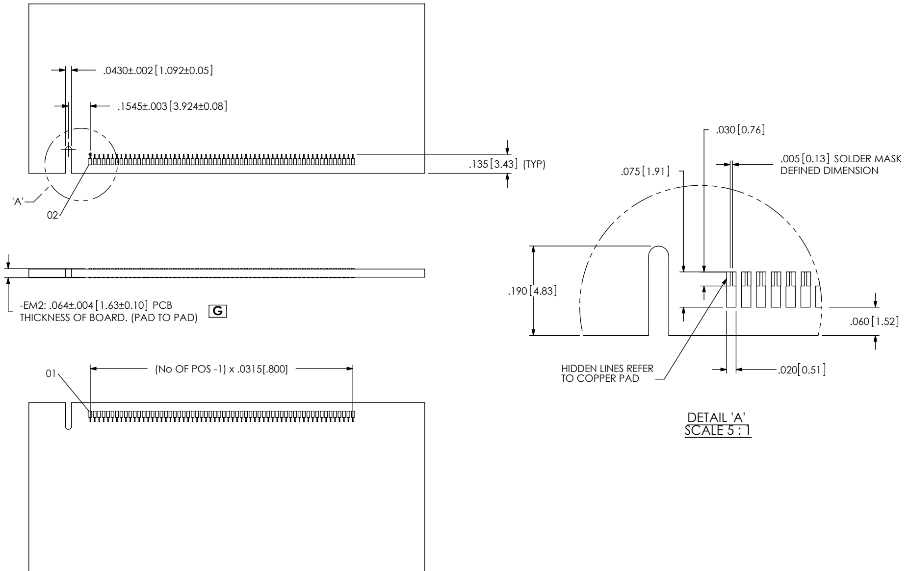
FIG 1: RECOMMENDED PCB LAYOUT FOR STANDARD DESIGNS
