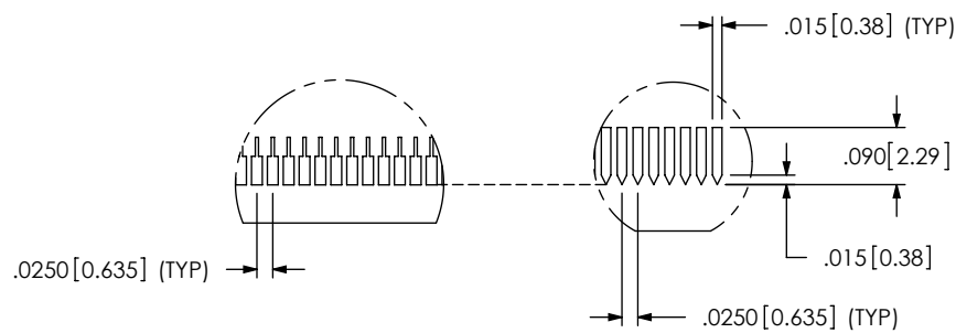
DETAIL 'C' SCALE 3:1 PCB VIEW
