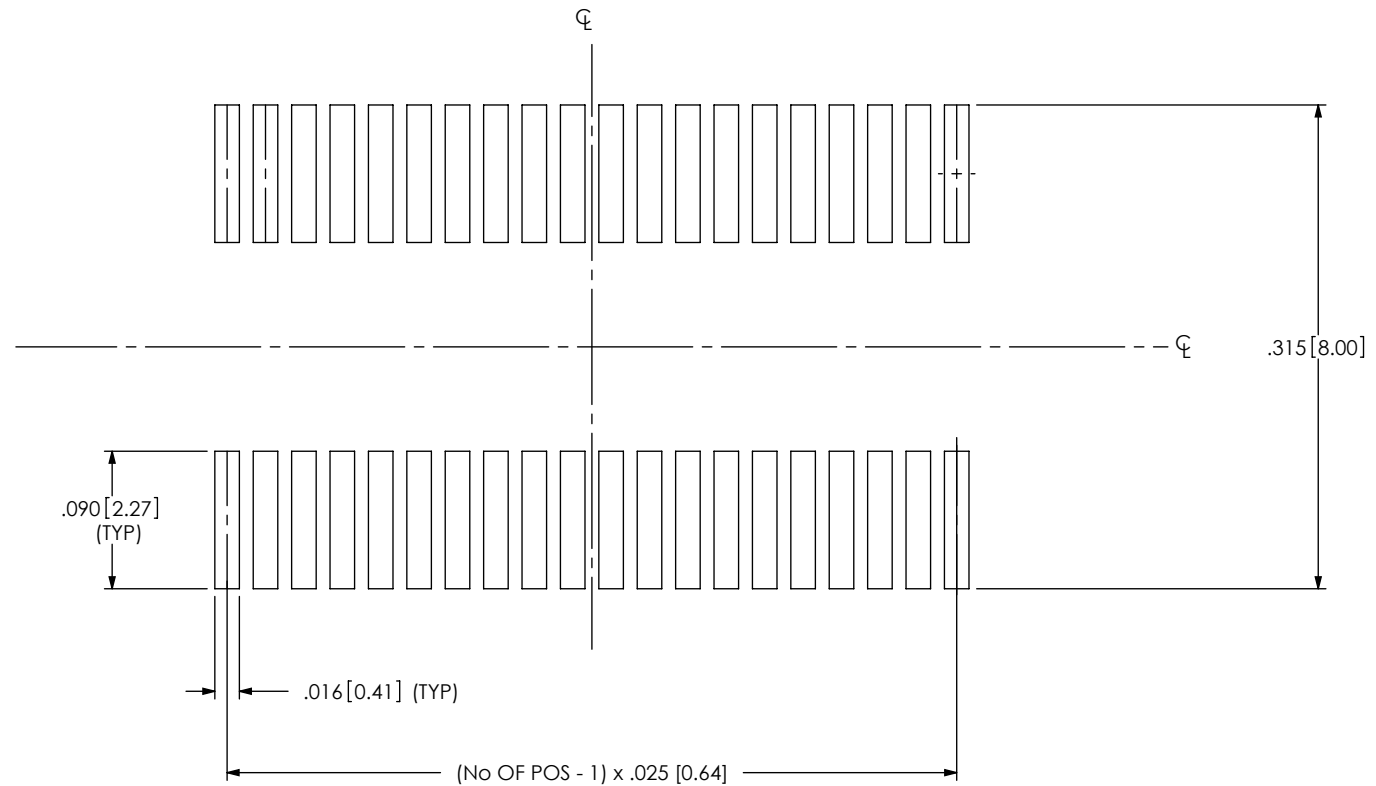
FIG 2 BSS-020-01-X-D SHOWN ALL DIMENSIONS ARE SYMMETRIC ABOUT THE CENTERLINE
