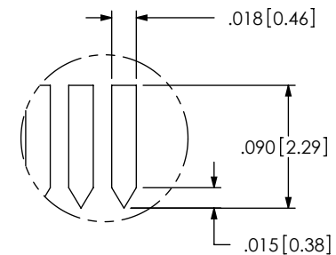
DETAIL 'C' SCALE 8 : 1
