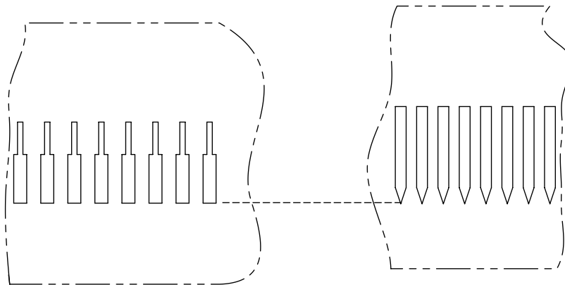
STENCIL DETAIL
