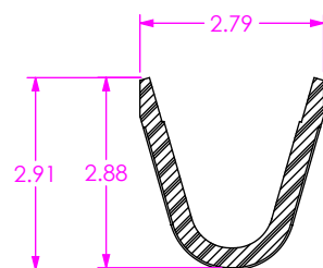
SECTION "A"-"A" SCALE 8 : 1
