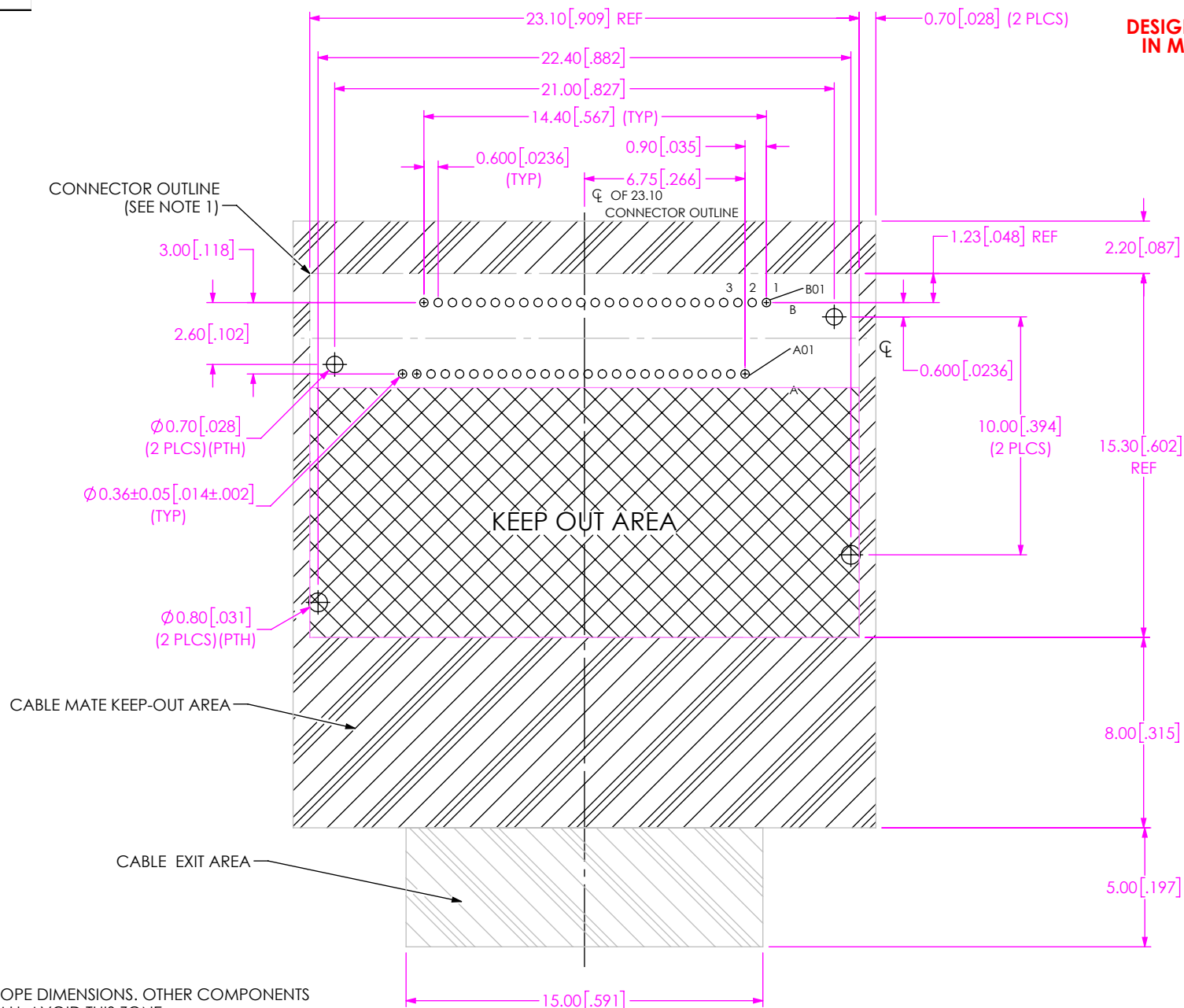
FIG 1 CPI-16-01-2-X-RA-X-L-XR FOOTPRINT SHOWN
