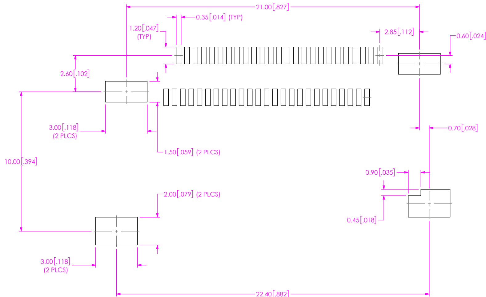
FIG 2 CPI-01-01-2-X-RA-X-L-X-XR STENCIL SHOWN (DIFFERENT AS SHOWN, OTHERWISE SAME AS FIG 1)
