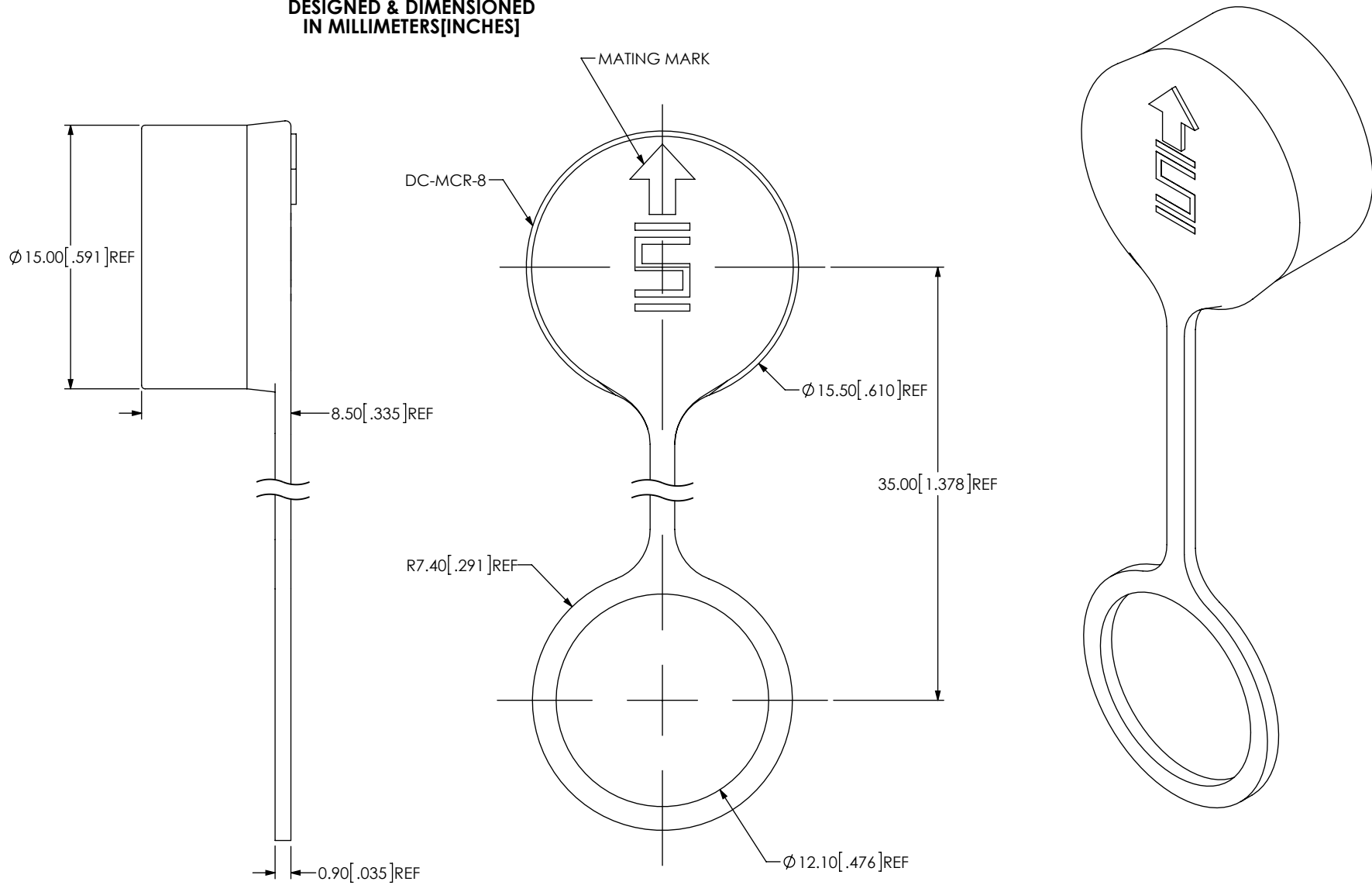
FIG 1 DCA-MCR-8 SHOWN
