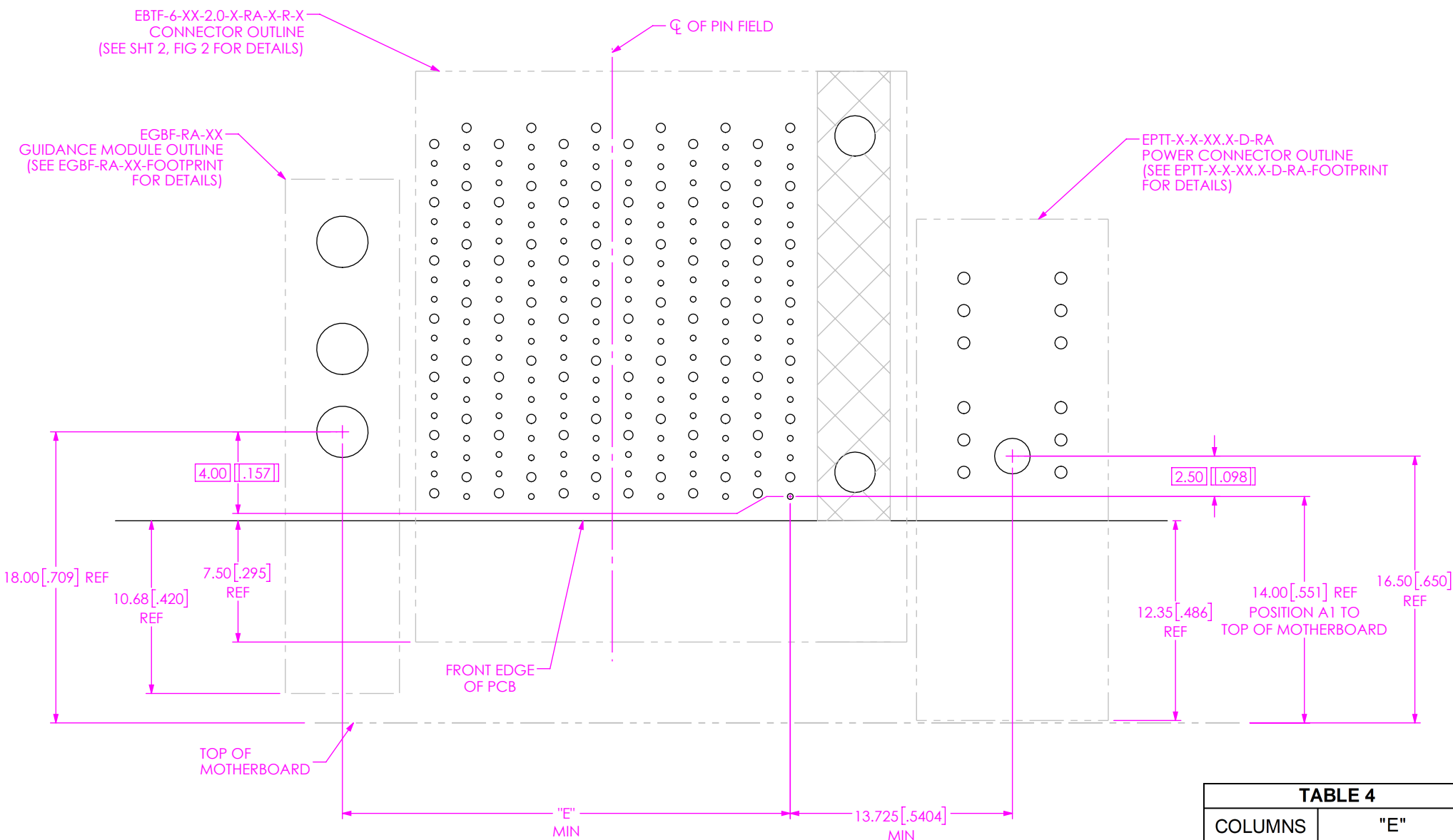
FIG 5 SIGNAL, POWER, INTERNAL (-R) AND EXTERNAL GUIDANCE COMBO EGBF-RA-XX-FOOTPRINT, EPTT-X-X-XX.X-D-RA-FOOTPRINT AND EBTF-6-12-2.0-X-RA-X-R-X-FOOTPRINT SHOWN
