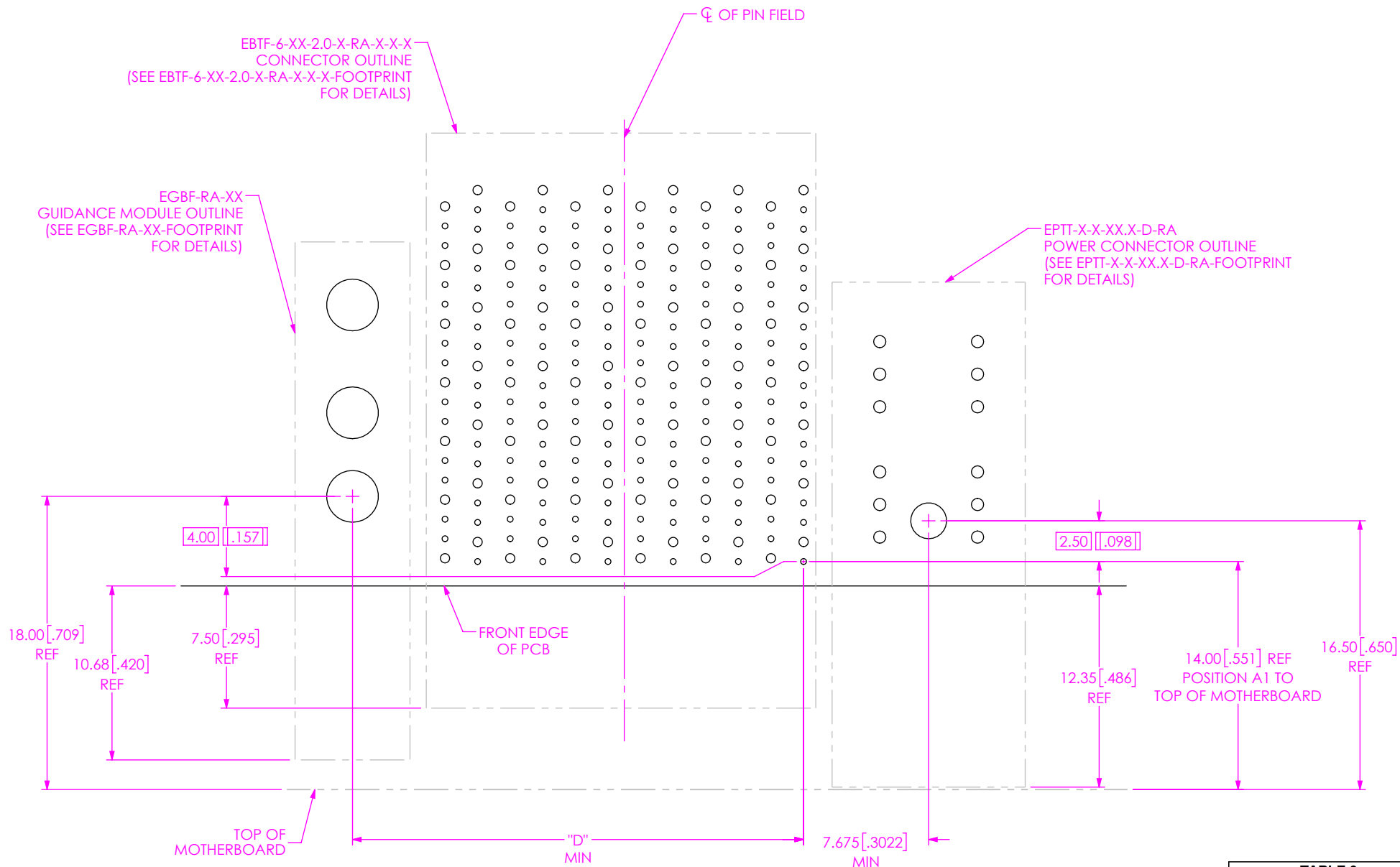
FIG 4 SIGNAL, POWER AND GUIDANCE COMBO EGBF-RA-XX-FOOTPRINT, EPTT-X-X-XX.X-D-RA-FOOTPRINT AND EBTF-6-12-2.0-X-RA-X-X-X-FOOTPRINT SHOWN
