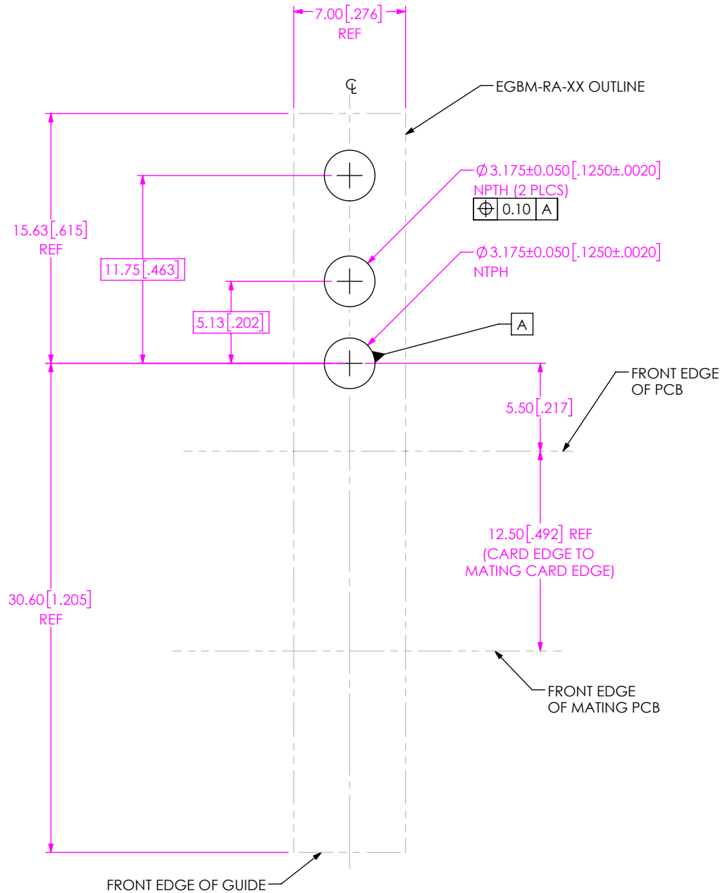
FIG 1 (SUGGESTED PCB LAYOUT) (COMPONENT SIDE SHOWN)
