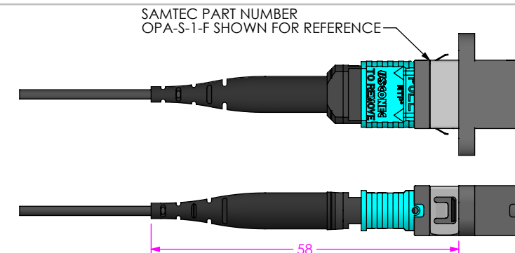
-7/-8 FIBER TYPE, -01/-02 END OPTION MATED WITH BULKHEAD DUST CAPS/PLUGS NOT SHOWN FOR CLARITY
