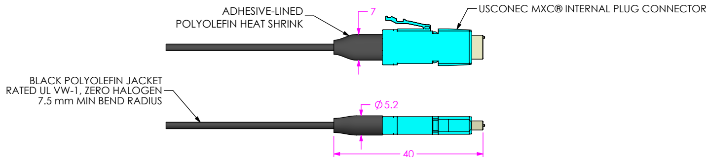
-7/-8 FIBER TYPE, -07 END OPTION DUST CAPS/PLUGS NOT SHOWN FOR CLARITY
