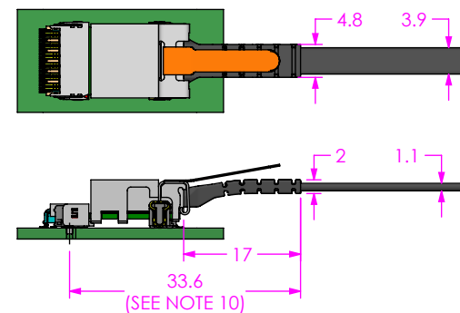
-5 FIBER TYPE, > 50 cm LENGTH
