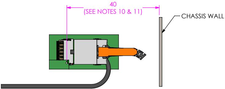
-7 FIBER TYPE RECOMMENDED CABLE ESCAPE CLEARANCE
