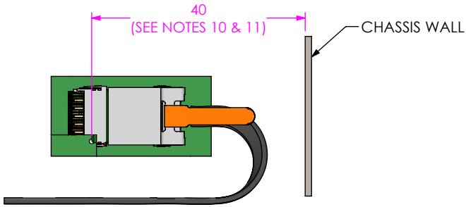
-6 FIBER TYPE RECOMMENDED CABLE ESCAPE CLEARANCE
