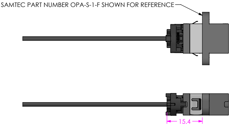
-7/-8 FIBER TYPE -0E END OPTION MATED WITH BULKHEAD
