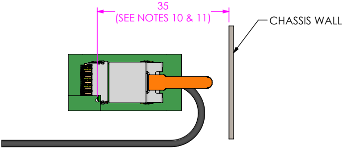
-8 FIBER TYPE RECOMMENDED CABLE ESCAPE CLEARANCE
