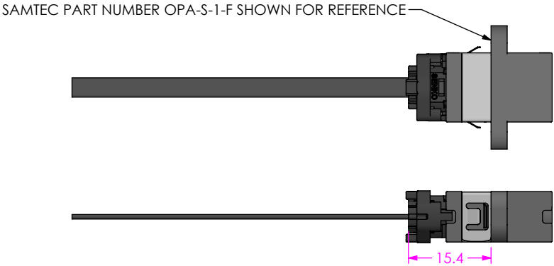
-5/-6 FIBER TYPE -0E END OPTION MATED WITH BULKHEAD
