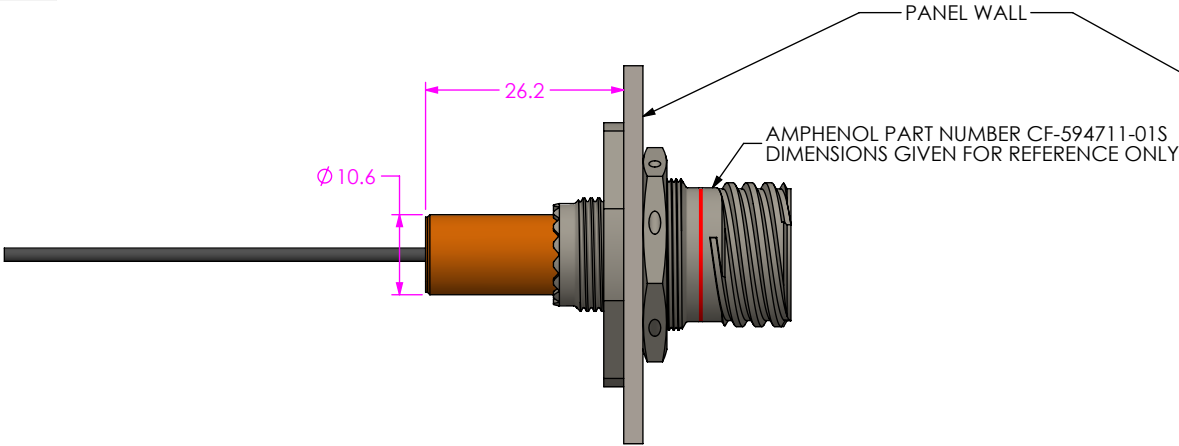
-7/-8 FIBER TYPE -0C END OPTION (SHOWN WITH PANEL)
