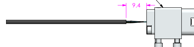
-7/-8 FIBER TYPE, -0A END OPTION WITH VITA 66.4 INSTALLED DUST CAPS/PLUGS NOT SHOWN FOR CLARITY
