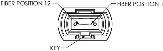
VIEW "A"- "A" END OPTIONS -01/-02/-0E
