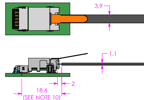
-6 FIBER TYPE, > 50 cm LENGTH
