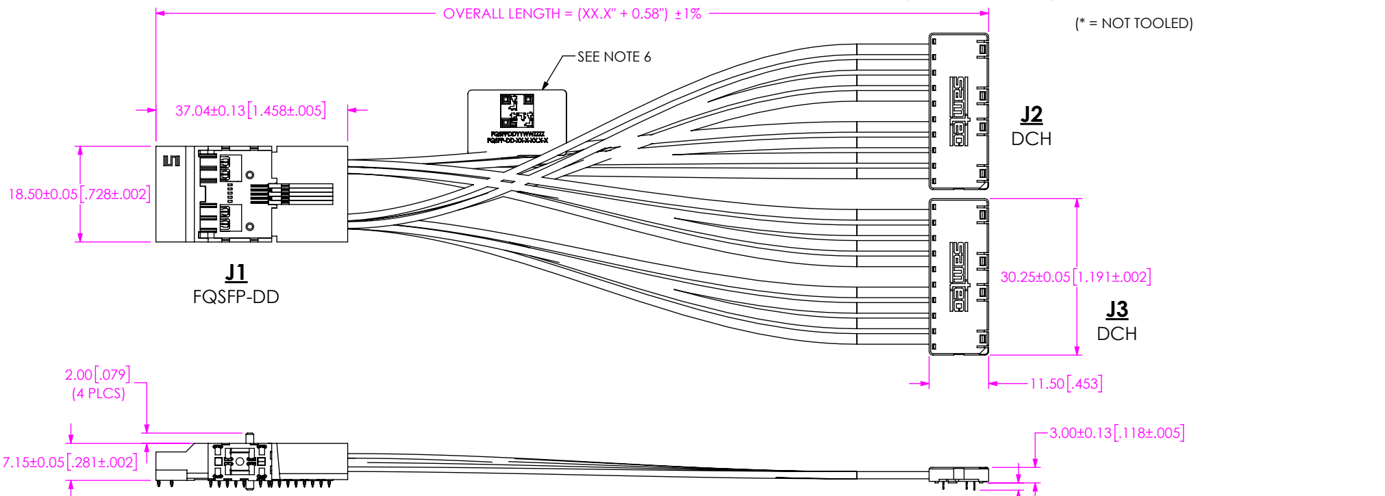
FIG 1 FQSFP-DD-01-A-06.0-1 SHOWN
