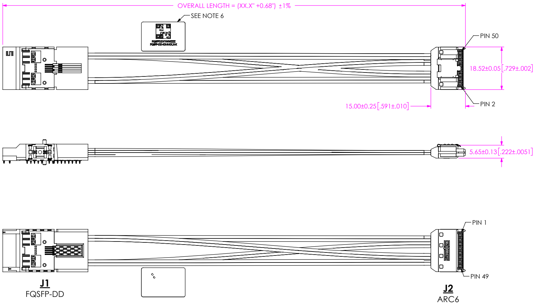
FIG 4 FQSFP-DD-01-A-06.0-3 SHOWN (SAME AS FIG 2, EXCEPT AS SHOWN)
