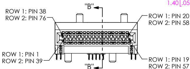
FIG 1 FQSFP-DD-01-A-06.0-1 SHOWN
