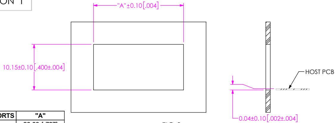
FIG 8 RECOMMENDED PANEL OPENING FOR QSFP-DD-X-X-X-XX-F
