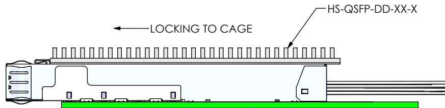
FIG 12 HEAT SINK LOCK
