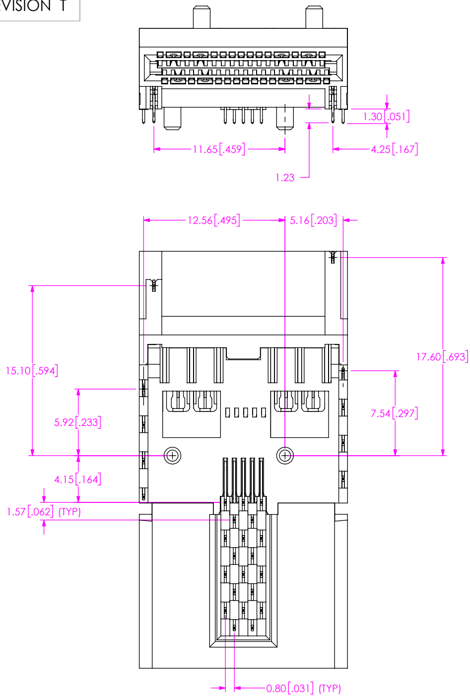
FIG 6 FQSFP-DD-01-A-XX.X-X BOTTOM SHOWN
