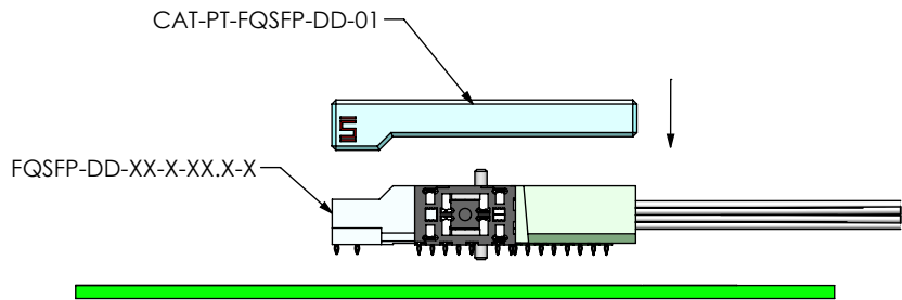
FIG 10 CONNECTOR PRESS
