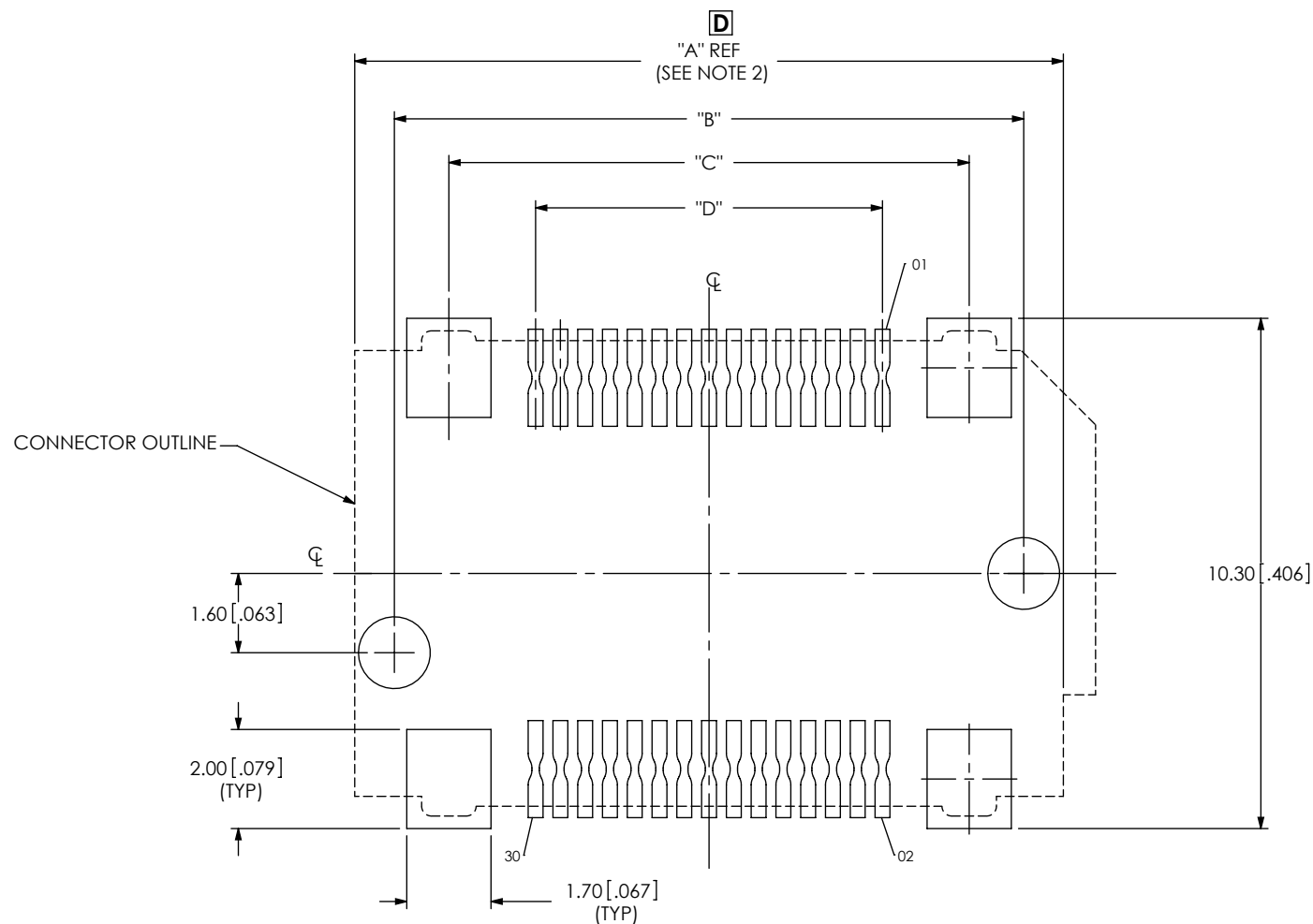
FIG 3 -SM OPTION (SAME AS FIG 1, EXCEPT AS SHOWN) (FS5-15-04.0-X-DV-SM-X-TR PCB LAYOUT SHOWN) D
