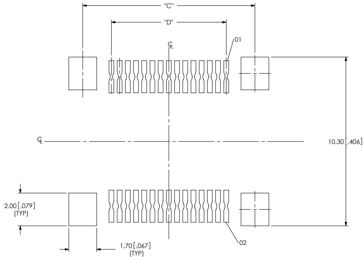
FIG 4 -SM OPTION (SAME AS FIG 2, EXCEPT AS SHOWN) (FS5-15-04.0-X-DV-SM-X-TR STENCIL SHOWN) D
