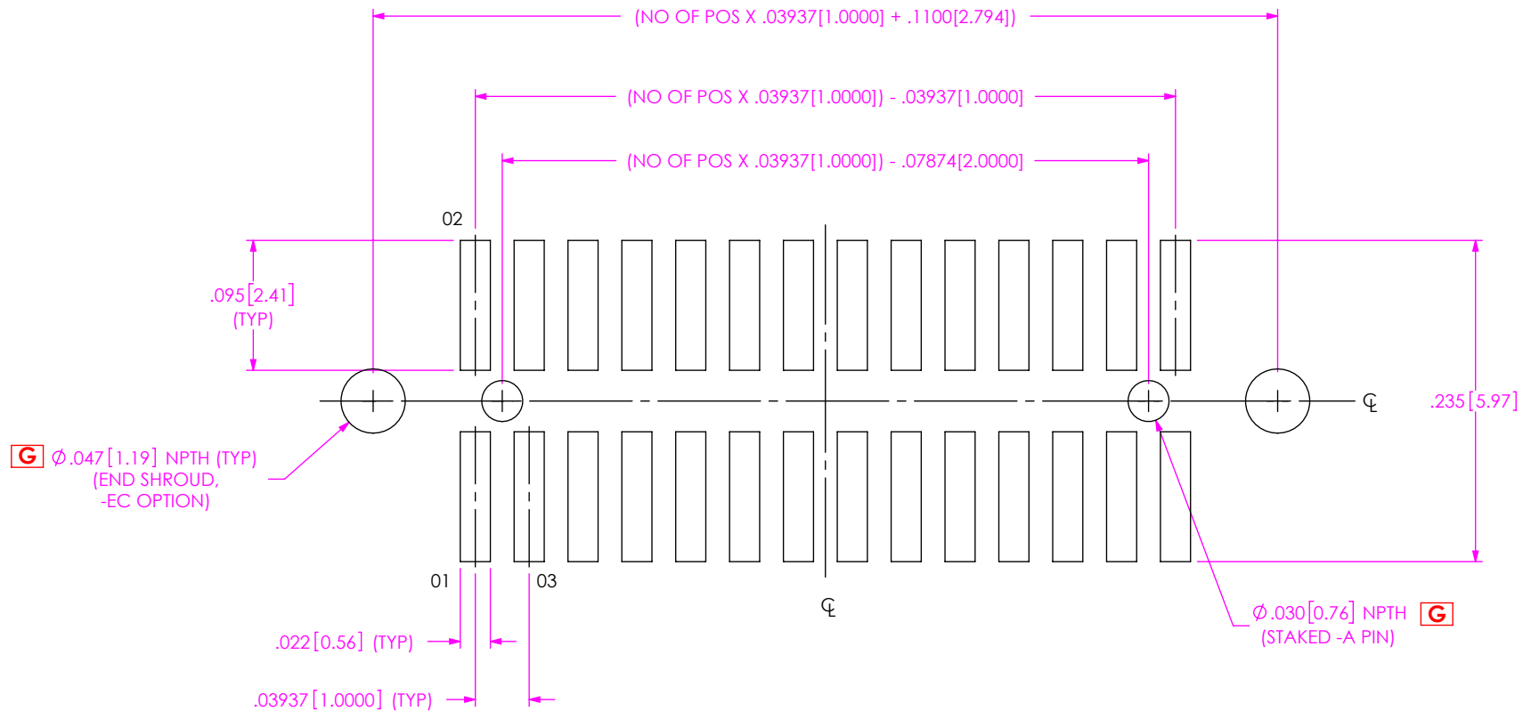
FIG 1 ALL DIMENSIONS ARE SYMMETRIC ABOUT THE CENTERLINE
