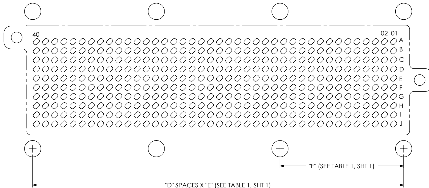
FIG 2 GMI-40-2-1.27-X-10 BOTTOM MATING BOARD SHOWN (DIFFERENT AS SHOWN, OTHERWISE SAME AS FIG 1) (NOT TOOLED)
