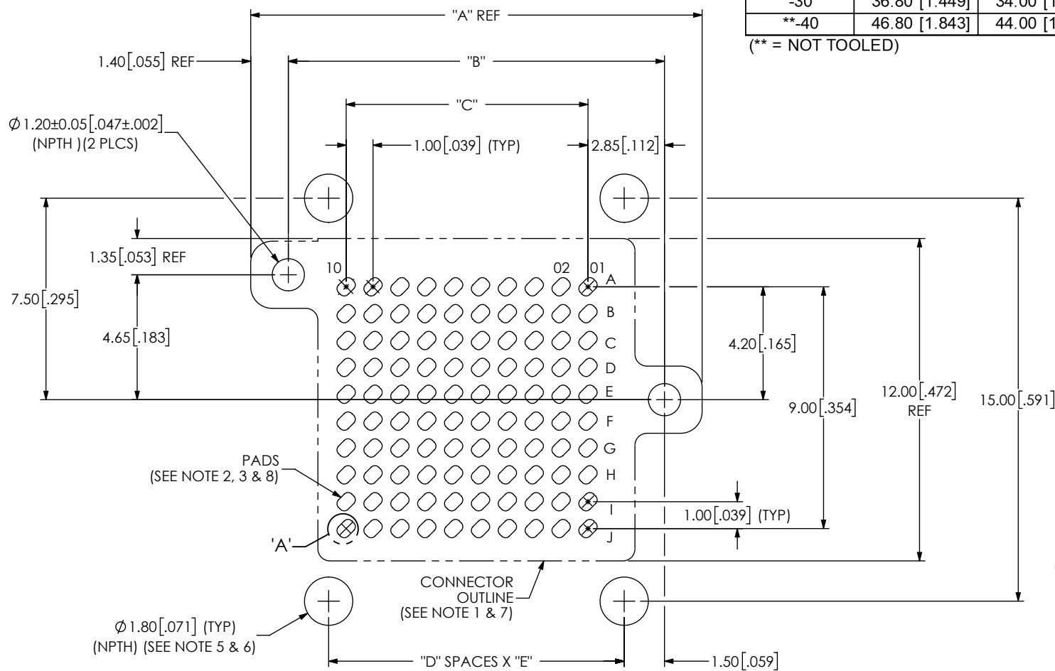
FIG 1 GMI-10-2-1.27-X-10 BOTTOM MATING BOARD SHOWN
