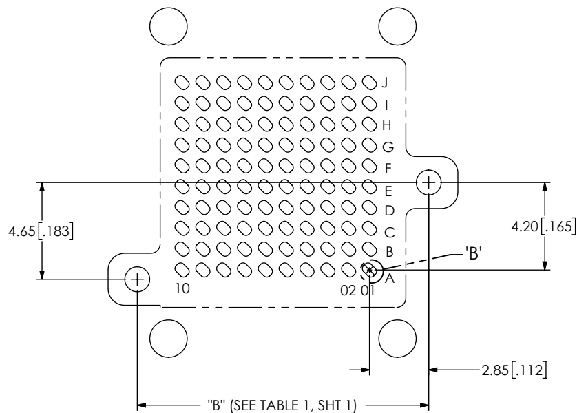
FIG 3 GMI-10-2-1.27-X-10 TOP MATING BOARD SHOWN (DIFFERENT AS SHOWN, OTHERWISE SAME AS FIG 1)
