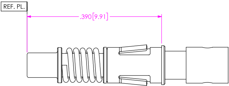
FIG. 2 SCALE 6:1 (OPERATING LENGTH) (ALL DIMS. SAME AS FIG. 1 UNLESS SHOWN)
