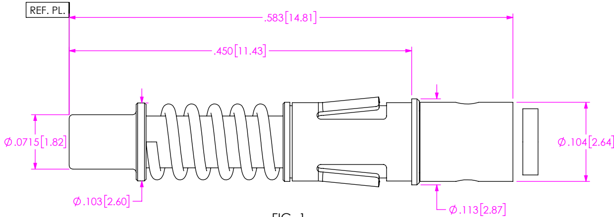
FIG. 1 (FREE LENGTH)
