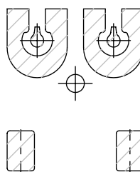
RECOMMENDED "-02" FOOTPRINT (GPPC-XX-1-02-XX-RA-SM SHOWN) (SAME AS ABOVE FOOTPRINT UNLESS OTHERWISE SHOWN.)
