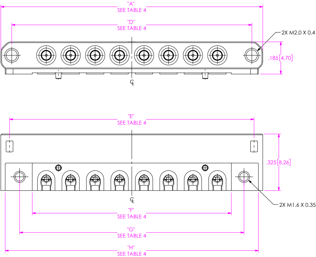
FIG 4 (GPPC-PF-1-08-XX-RA-SM-S-X SHOWN) (SAME AS FIG 1, EXCEPT AS SHOWN)
