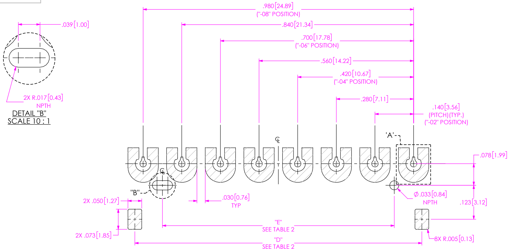
RECOMMENDED FOOTPRINT (GPPC-XX-1-08-XX-RA-SM SHOWN)
