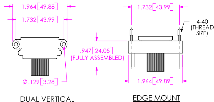
DUAL VERTICAL
