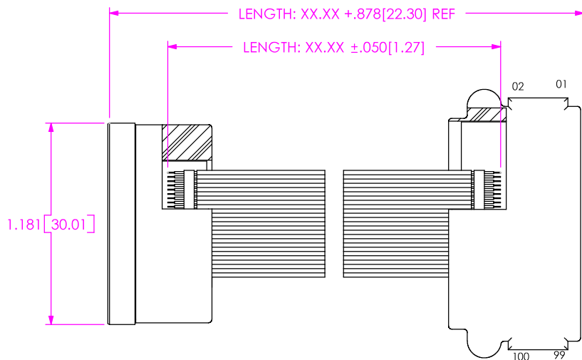
SECOND END
