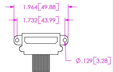
DUAL VERTICAL
