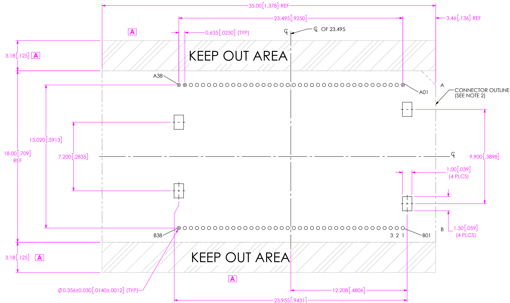
FIG 1 HLF6-38-03.5-XXX-2-XR FOOTPRINT SHOWN
