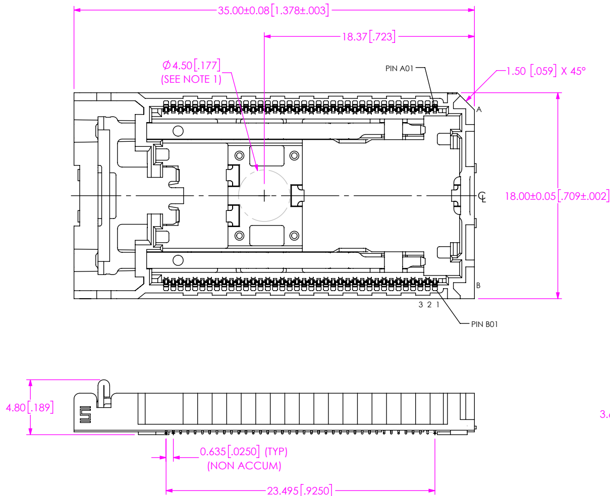
FIG 1 HLF6-38-03.5-XXX-2-XR SHOWN
