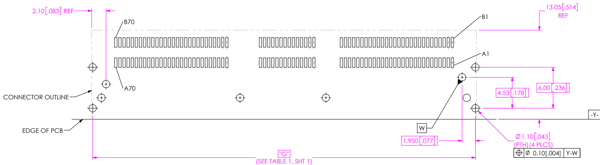
FIG 3 HSEC6-070-01-X-RA-S-WT-XR FOOTPRINT SHOWN (DIFFERENT AS SHOWN, OTHERWISE SAME AS FIG 1) (FOR -028, -042 & -070 POS ONLY)
