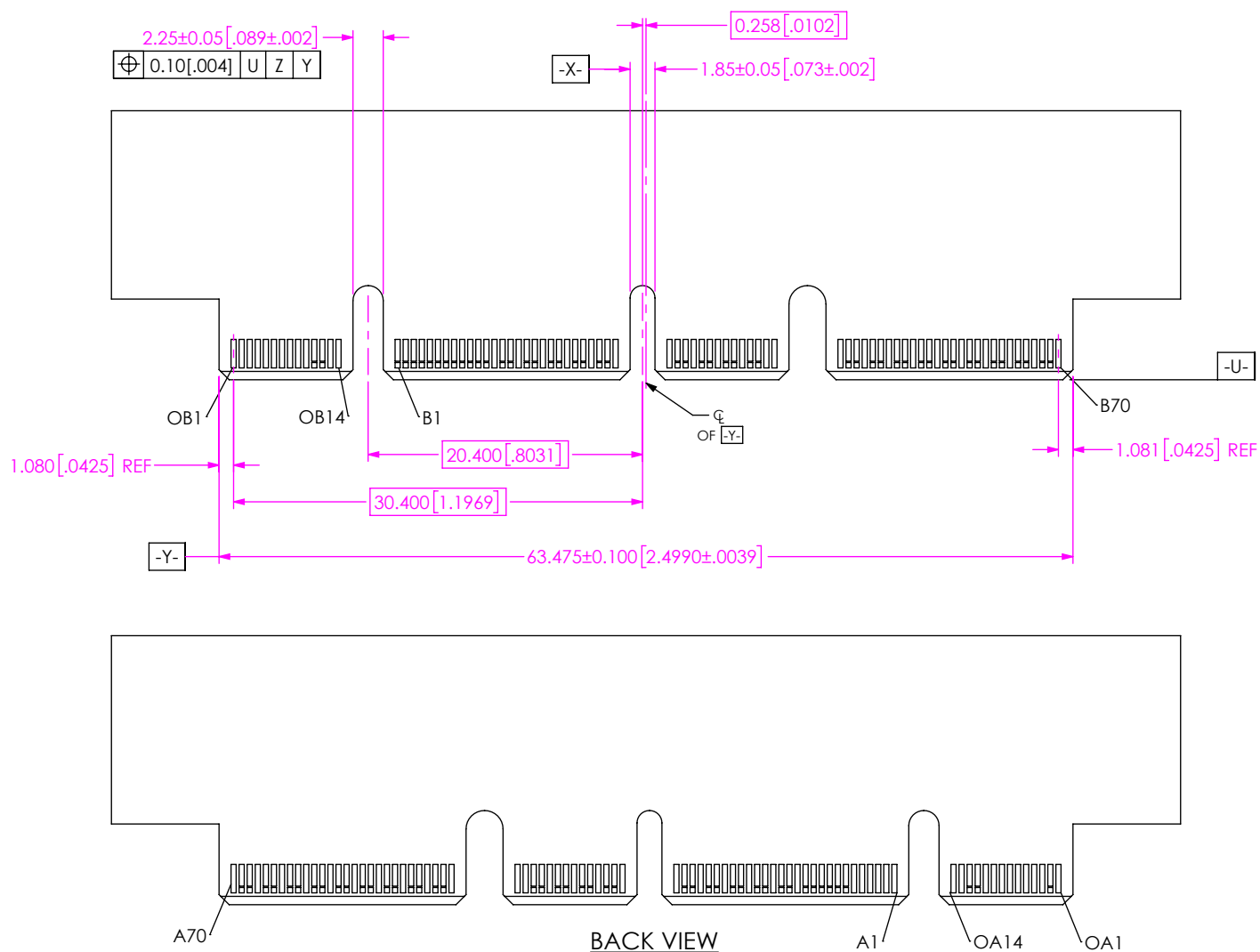
FIG 12 HSEC6-084-01-X-RA-WT-XR MATING CARD SHOWN (DIFFERENT AS SHOWN, OTHERWISE SAME AS FIG 9) (FOR -084 POS ONLY)
