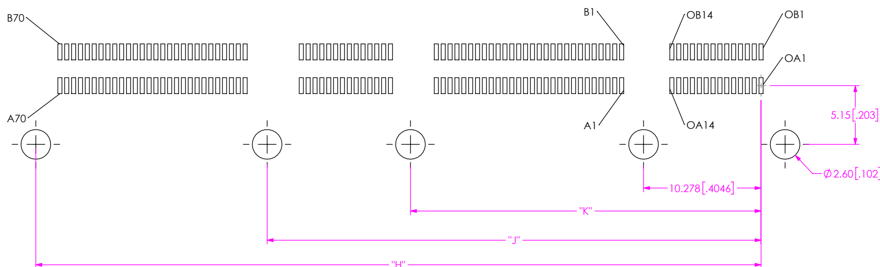
FIG 6 HSEC6-084-01-X-RA-WT-XR STENCIL SHOWN (DIFFERENT AS SHOWN, OTHERWISE SAME AS FIG 2 & 3) (FOR -084 POS ONLY)
