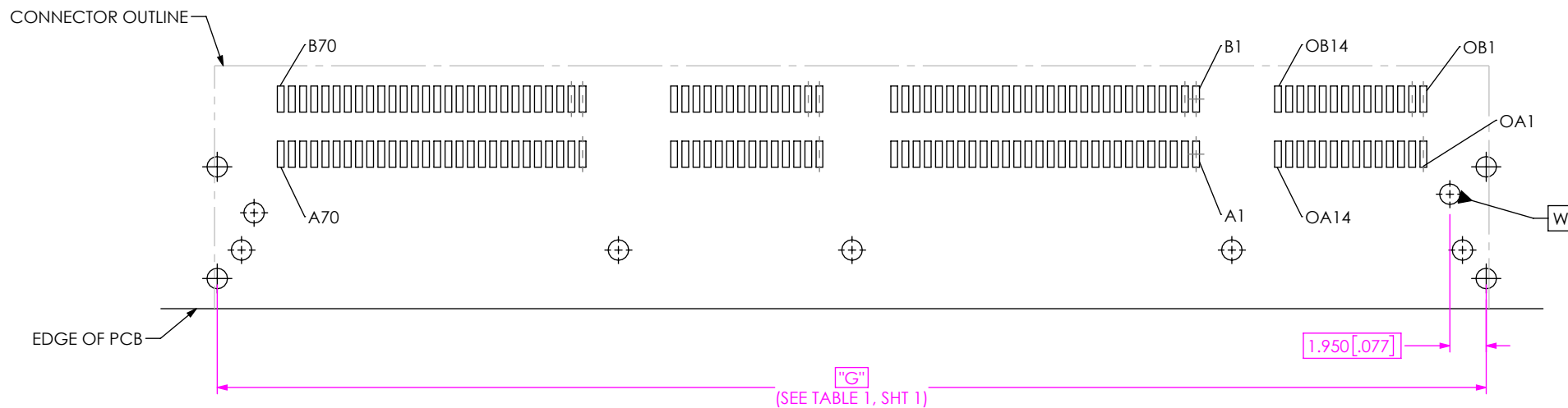
FIG 4 HSEC6-084-01-X-RA-S-WT-XR FOOTPRINT SHOWN (DIFFERENT AS SHOWN, OTHERWISE SAME AS FIG 2 & 3) (FOR -084 POS ONLY)
