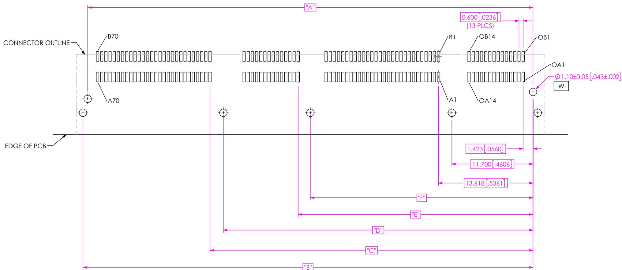
FIG 2 HSEC6-084-01-X-RA-WT-XR FOOTPRINT SHOWN (DIFFERENT AS SHOWN, OTHERWISE SAME AS FIG 1) (FOR -084 POS ONLY)
