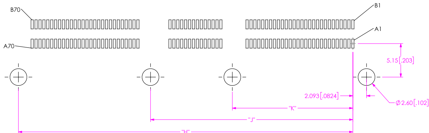
FIG 5 HSEC6-070-01-X-RA-WT-XR STENCIL SHOWN (DIFFERENT AS SHOWN, OTHERWISE SAME AS FIG 1) (FOR -028, -042 & -070 POS ONLY)
