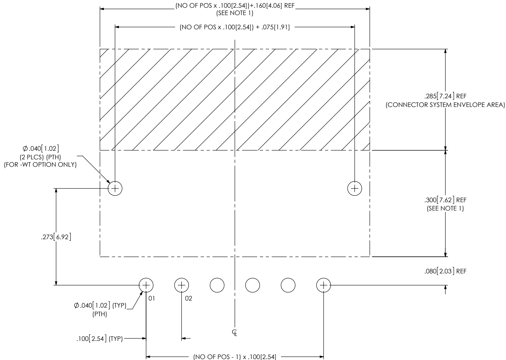
FIG 1 IPL1-106-01-XXX-S-RE1-K-WT SHOWN
