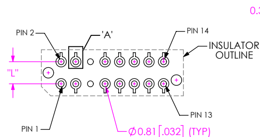
FIG 4 MEC2-08-02-X-THX-XX FOOTPRINT SHOWN (SAME AS FIG 1, EXCEPT AS SHOWN)
