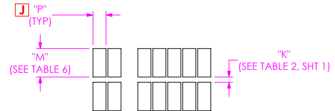
FIG 8 MEC2-08-01-X-THX-XX STENCIL SHOWN (SAME AS FIG 5, EXCEPT AS SHOWN)
