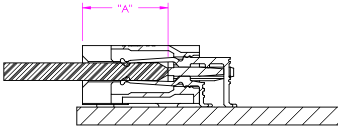
SECTION "A"- "A" SCALE 3 : 1
