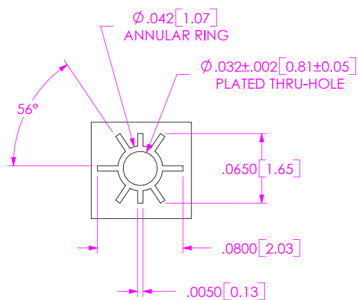
DETAIL "A" SCALE 8 : 1
