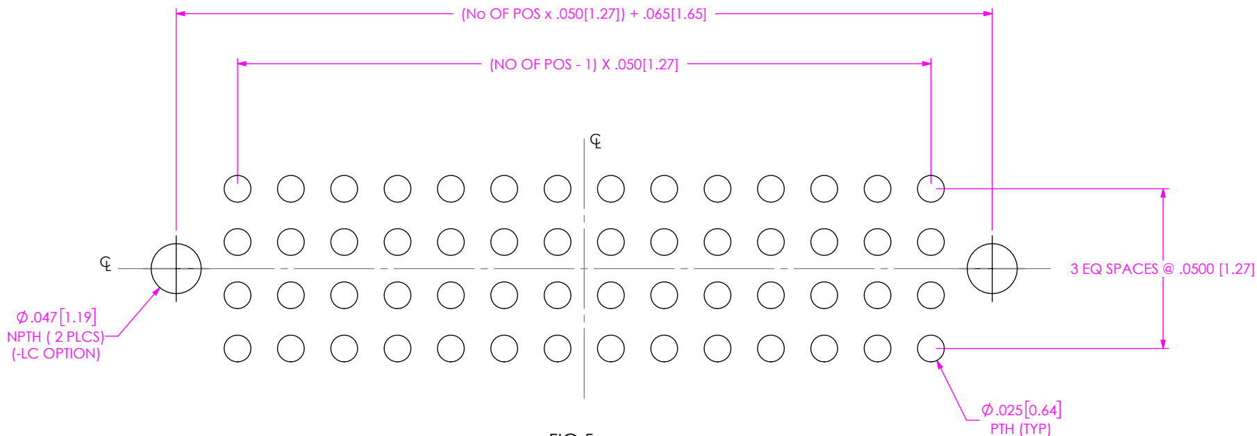
FIG 5 MOLC-114-XX-XX-Q-LC SHOWN (ALL DIMENSIONS ARE SYMMETRICAL ABOUT THE CENTERLINE)
