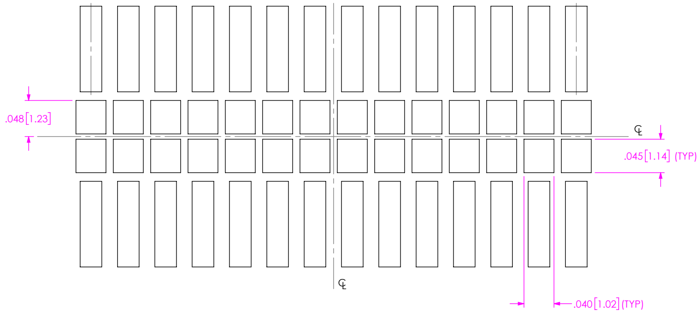
FIG 2 MOLC-114-M1-XX-Q-LC SHOWN (SAME AS FIG 1, EXCEPT AS SHOWN)
