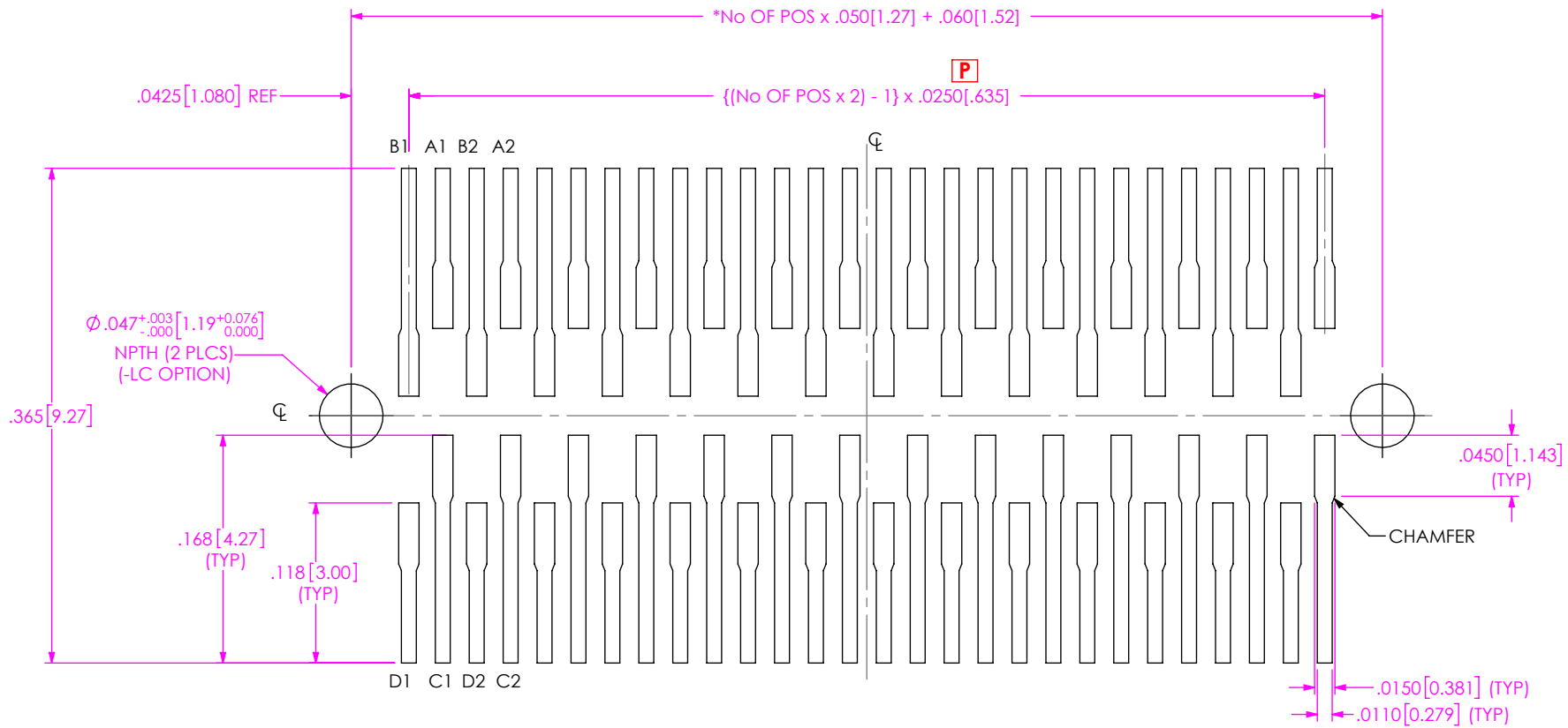
FIG 3 MOLC-114-02-XXX-Q-LC-XX SHOWN (ALL DIMENSIONS ARE SYMMETRICAL ABOUT THE CENTERLINE)
