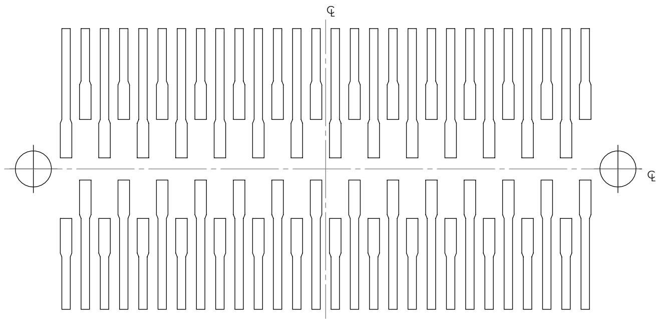
FIG 4 MOLC-114-02-XXX-Q-LC-XX SHOWN (SAME AS FIG 3)
