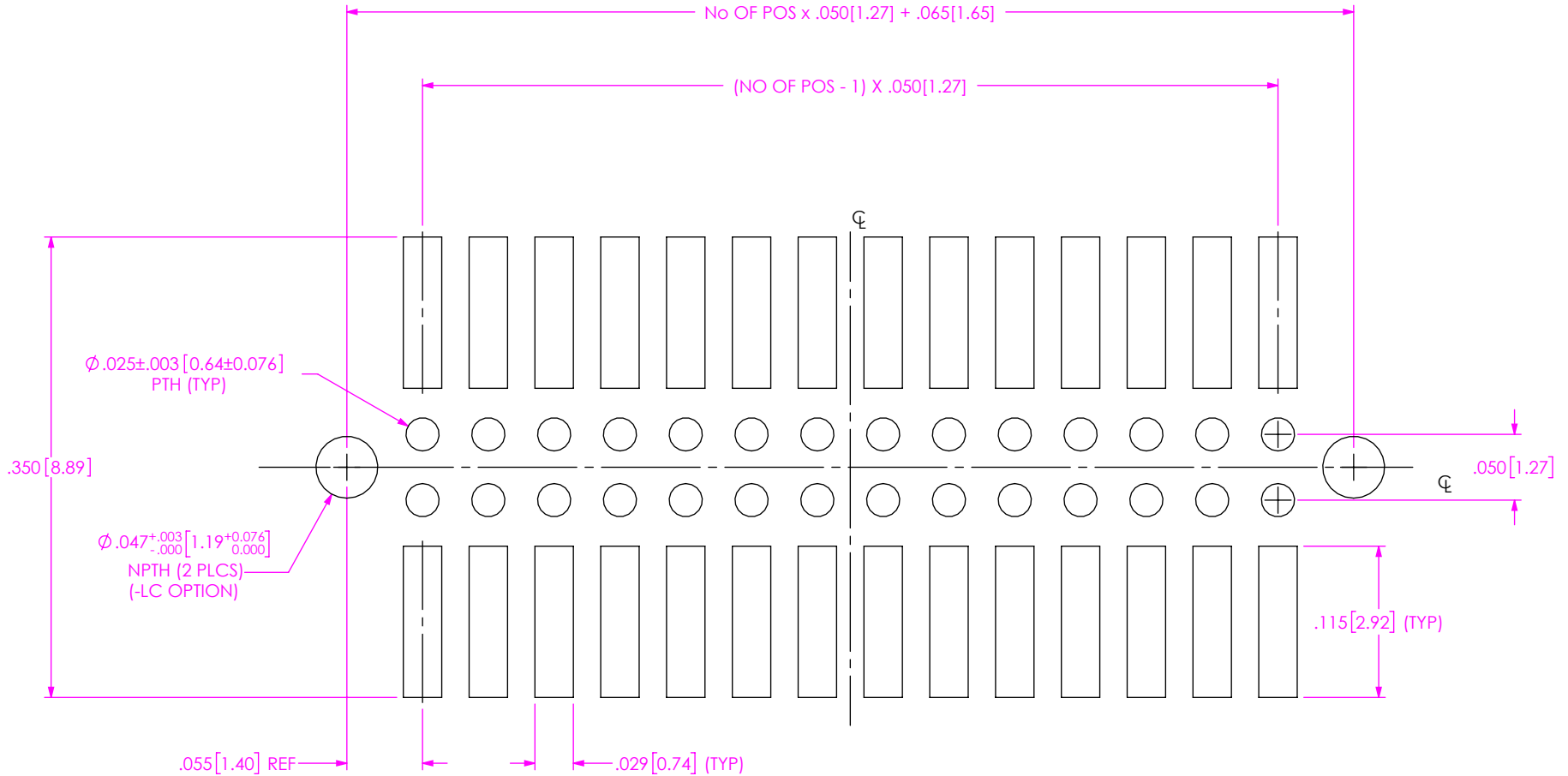
FIG 1 MOLC-114-M1-XX-Q-LC SHOWN (ALL DIMENSIONS ARE SYMMETRICAL ABOUT THE CENTERLINE)
