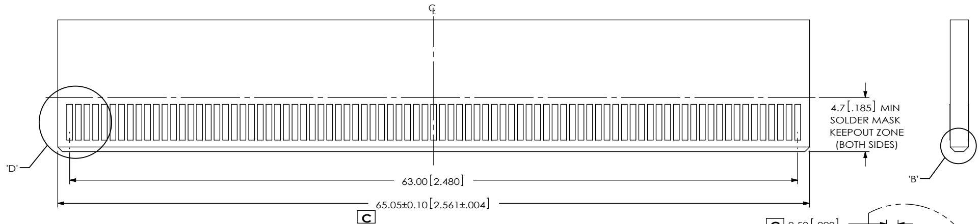
FIGURE 3 MTCA-085-XX-X-DV-SMT EDGE CARD SHOWN
