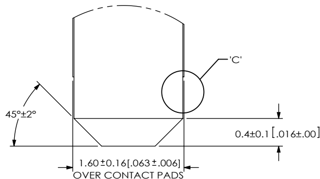
DETAIL 'B' SCALE 18:1
