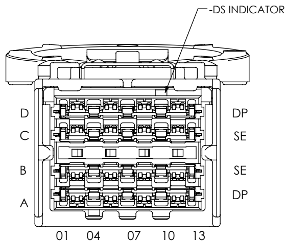
FIG 2 NVACE-DS-XX-4-X.X-A-X-1 (SAME AS FIG 1, EXCEPT AS SHOWN)
