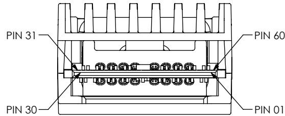
END 1 NOT SHOWN FOR CLARITY VIEW "H"-"H" (FOR -1: 34100 CABLE STYLE)
