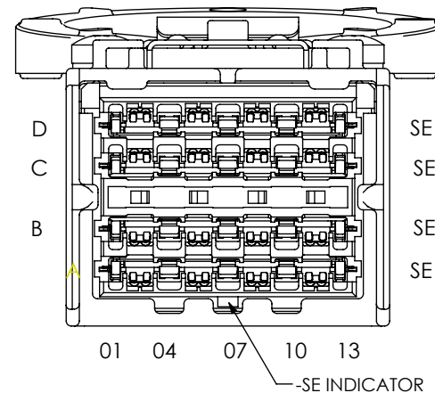
FIG 3 NVACE-SE-XX-4-X.X-A-X-1 (SAME AS FIG 1, EXCEPT AS SHOWN)
