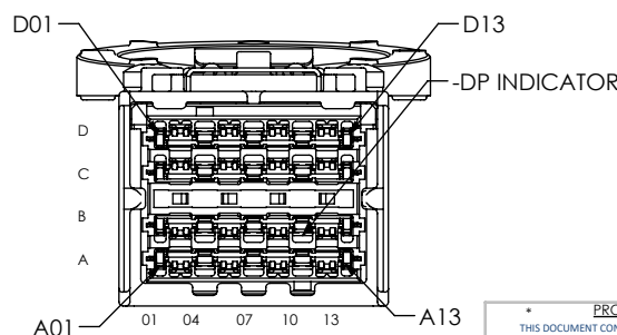
VIEW "B"- "B"
