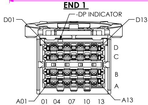
END 2 NOT SHOWN FOR CLARITY VIEW "G"-"G"
