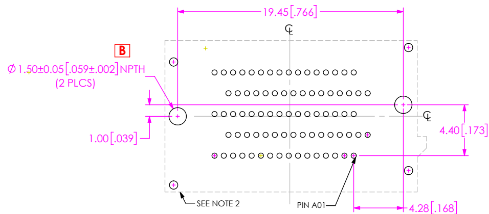
FIG 12 NVAM-DP-05-1-XX.X-X-X-CX (WITH A-PINS) FOOTPRINT SHOWN
