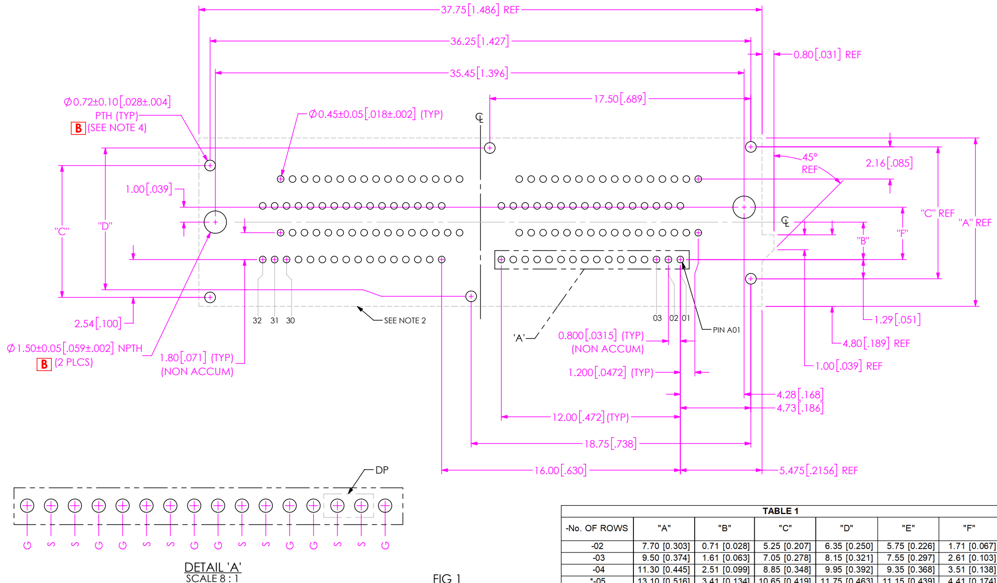
FIG 1 NVAM-DP-04-2-XX.X-X-X-CX FOOTPRINT SHOWN
