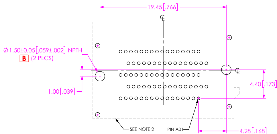
FIG 13 NVAM-DP-06-1-XX.X-X-X-CX (WITH A-PINS) FOOTPRINT SHOWN
