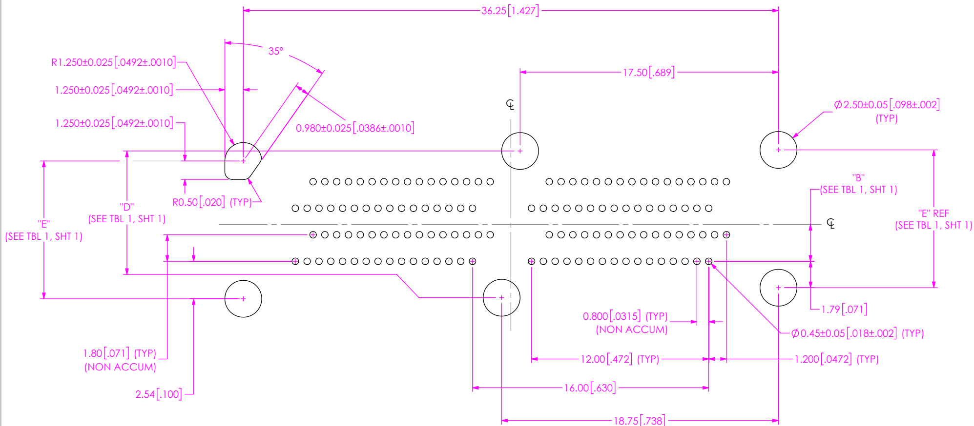
FIG 2 NVAM-DP-04-2-XX.X-X-X-CX STENCIL SHOWN
