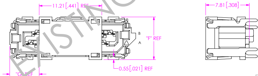
FIG 6 PICK AND PLACE PAD NVAM-DP-02-1-02.0-X-X-C-XR SHOWN
