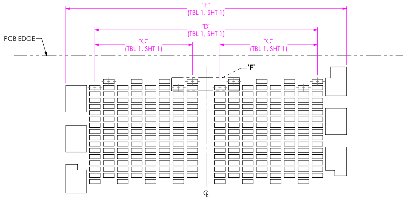
FIG 6 NVBM-XX-16-RA-XXX-0-XX STENCIL LAYOUT SHOWN (SAME AS FIG 2, EXCEPT AS SHOWN) (FOR -0 COLUMN OPTION ONLY)
