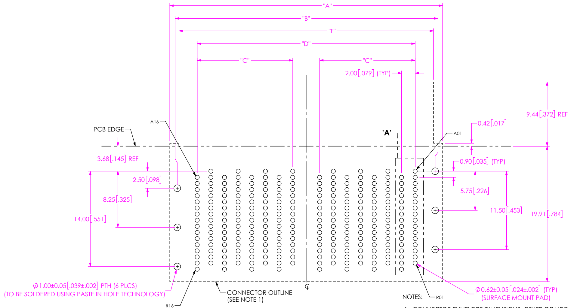
FIG1 NVBM-XX-16-RA-XXX-X-XX FOOTPRINT SHOWN
