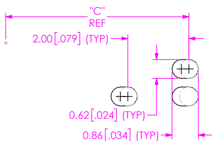
FIG 2 NVBM-XX-16-RA-XXX-2-XX STENCIL LAYOUT SHOWN (SAME AS FIG 1, EXCEPT AS SHOWN) (FOR -1, -2 SOLDER CHARGE OPTION ONLY)
