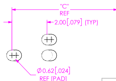
FIG 2 NVBM-XX-16-RA-XXX-2-XX STENCIL LAYOUT SHOWN (SAME AS FIG 1, EXCEPT AS SHOWN) (FOR -1, -2 SOLDER CHARGE OPTION ONLY)
