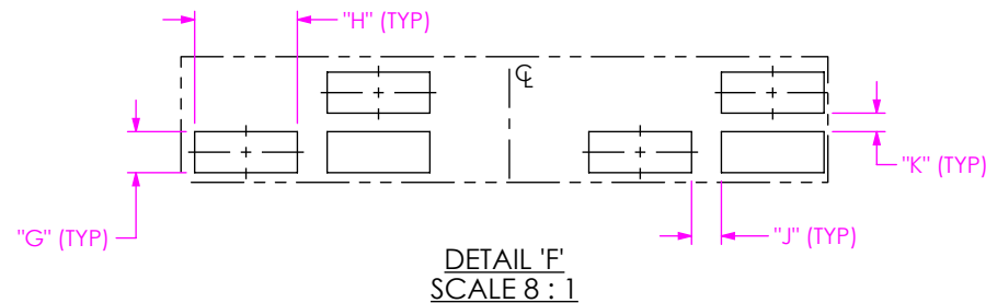
FIG 6 NVBM-XX-16-RA-XXX-0-XX STENCIL LAYOUT SHOWN (SAME AS FIG 2, EXCEPT AS SHOWN) (FOR -0 COLUMN OPTION ONLY)
