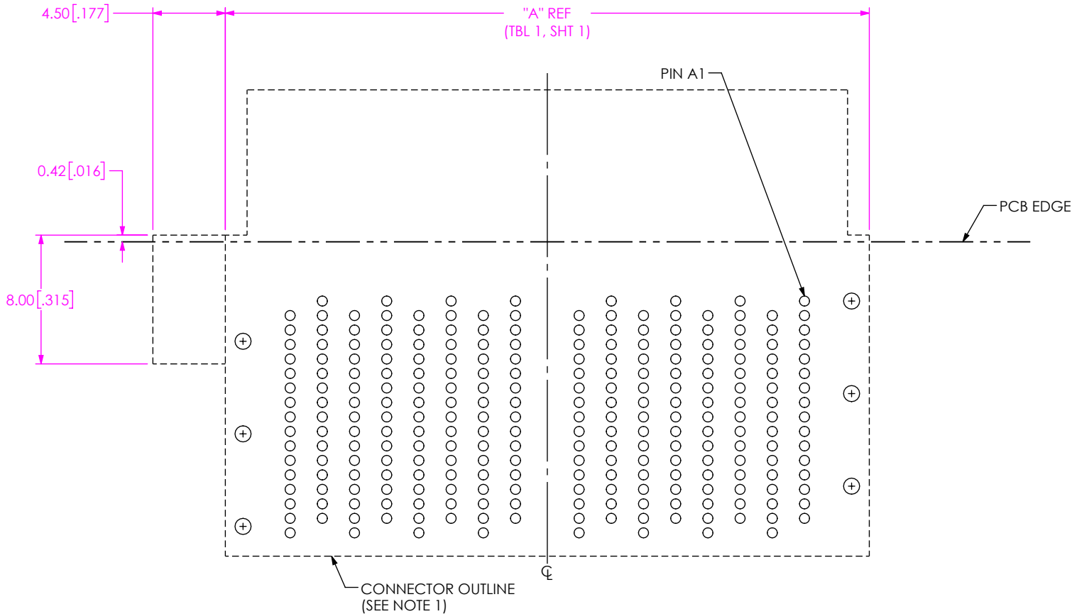
FIG 4 NVBM-XX-16-RA-XXX-R-X-XX FOOTPRINT SHOWN (SAME AS FIG 1, EXCEPT AS SHOWN)
