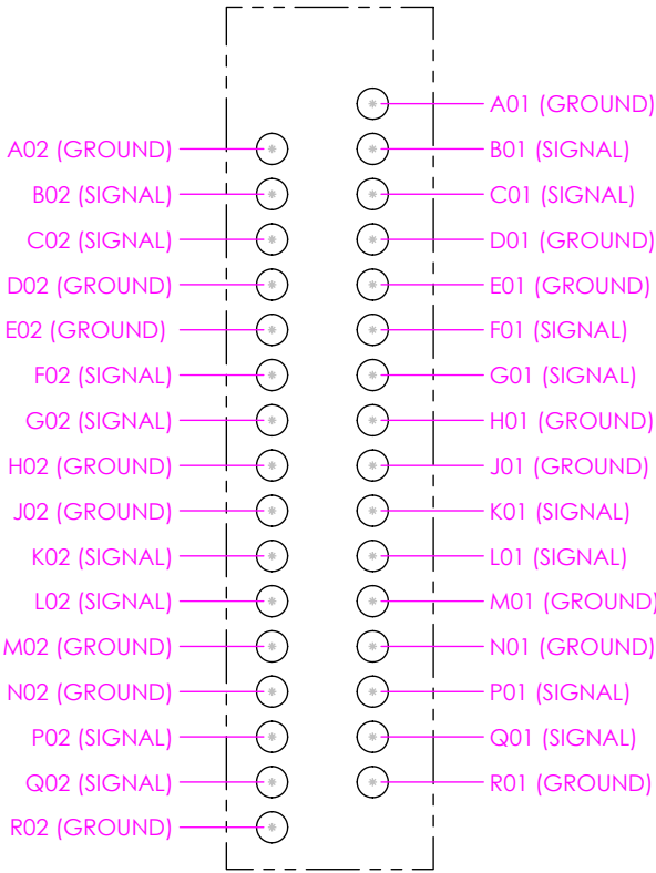
DETAIL 'A' SCALE 6:1 (PINOUT)
