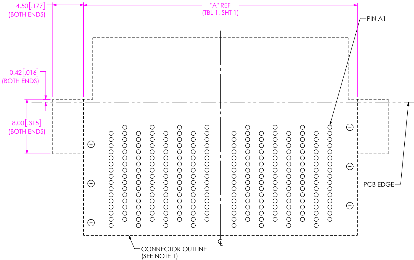
FIG 5 NVBM-XX-16-RA-XXX-B-X-XX FOOTPRINT SHOWN (SAME AS FIG 1, EXCEPT AS SHOWN)
