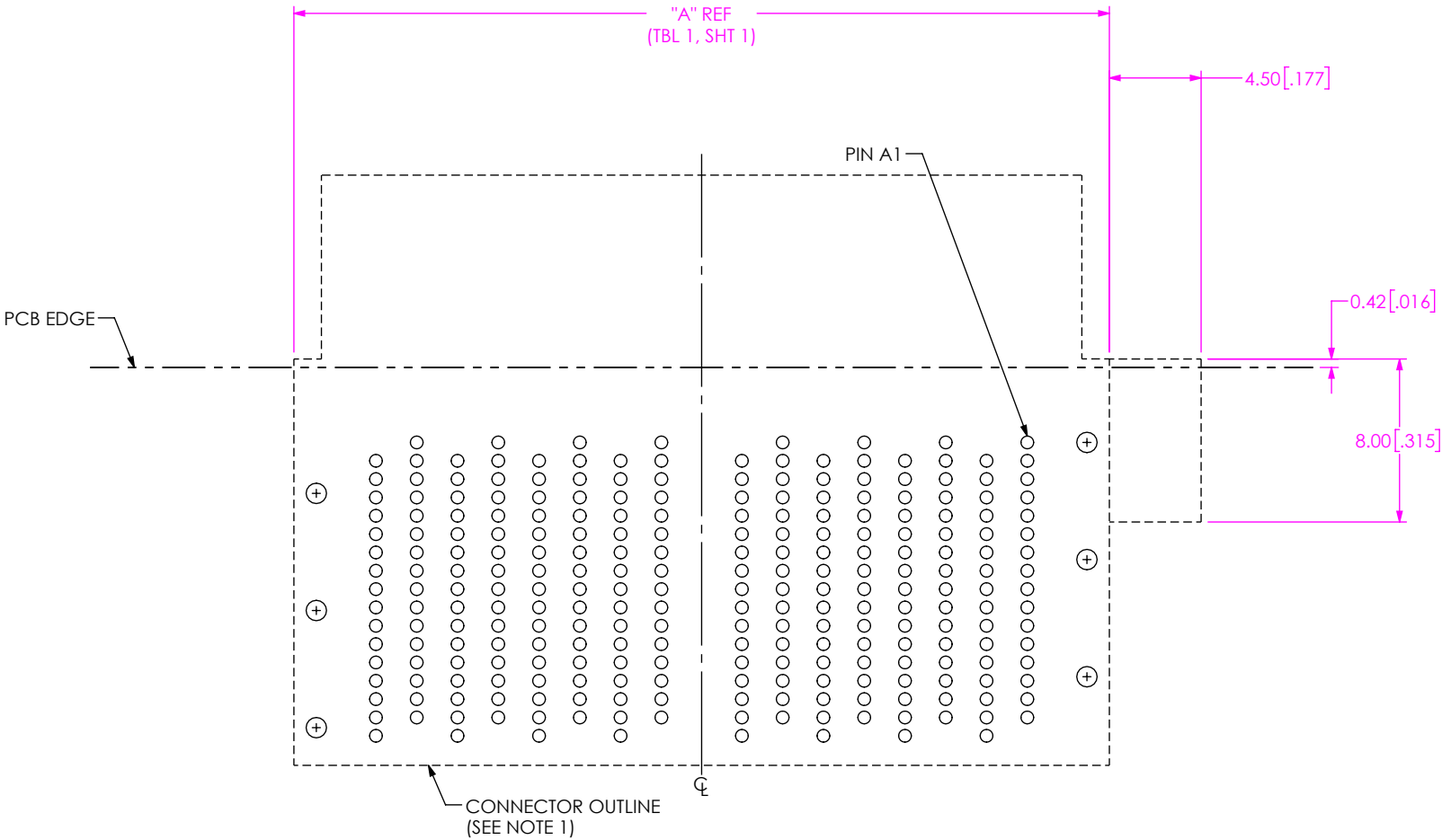
FIG 3 NVBM-XX-16-RA-XXX-L-X-XX FOOTPRINT SHOWN (SAME AS FIG 1, EXCEPT AS SHOWN)
