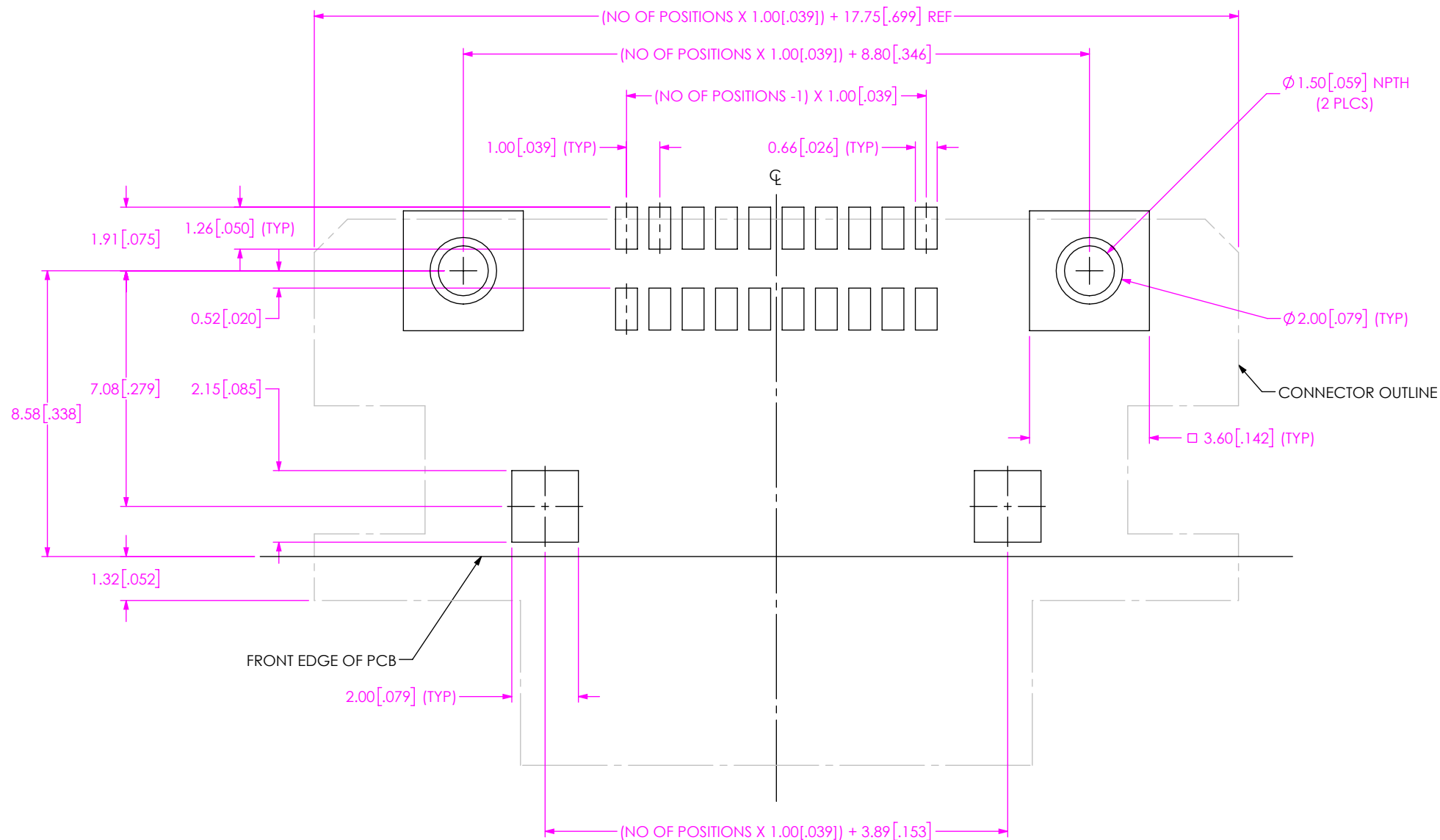
FIG 1 (-10 POSITION SHOWN) (P1M-XX-01-XXX-D-RA-XR PCB LAYOUT SHOWN) ALL DIMENSIONS ARE SYMMETRIC ABOUT THE CENTERLINE
