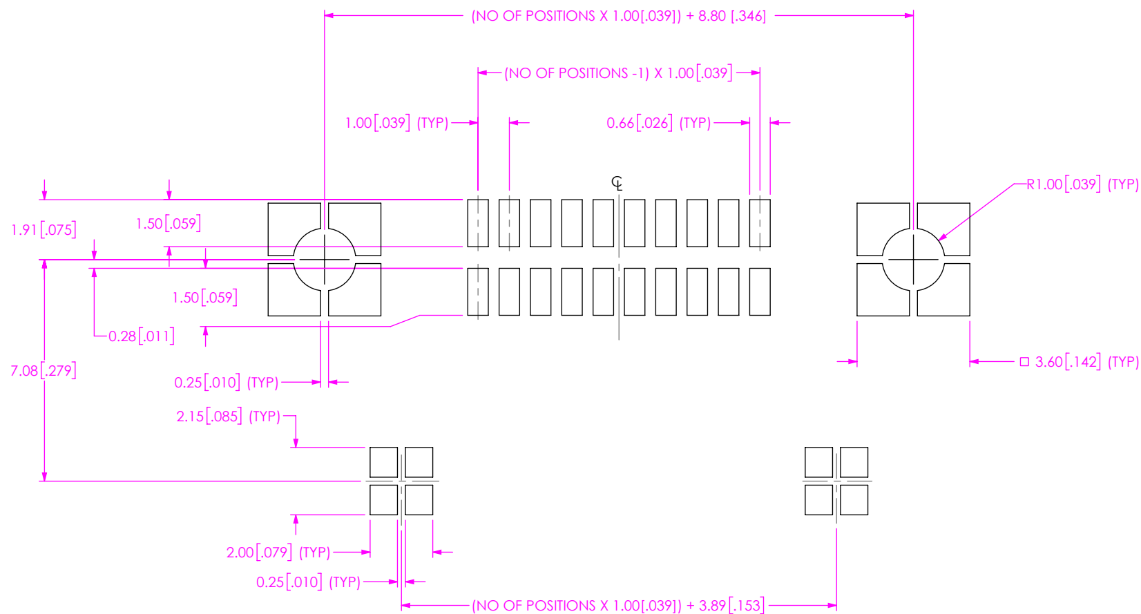
FIG 2 (-10 POSITION SHOWN) (P1M-XX-01-XXX-DV-XR STENCIL SHOWN) ALL DIMENSIONS ARE SYMMETRIC ABOUT THE CENTERLINE.
