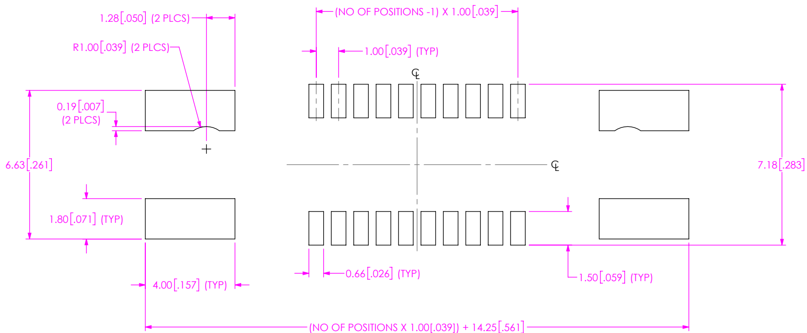
FIG 2 (-10 POSITION SHOWN) ( P1M-XX-01-XXX-DV-X STENCIL SHOWN) ALL DIMENSIONS ARE SYMMETRIC ABOUT THE CENTERLINE
