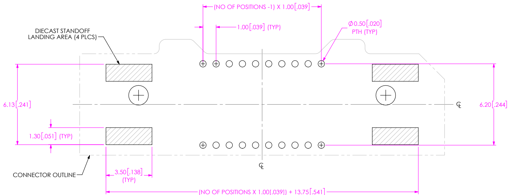
FIG 3 (-10 POSITION SHOWN) ( P1M-XX-02-XXX-DV-X & P1M-XX-03-XXX-DV-X PCB LAYOUT SHOWN) (DIFFERENCE AS SHOWN, OTHERWISE SAME AS FIG 1) ALL DIMENSIONS ARE SYMMETRIC ABOUT THE CENTERLINE
