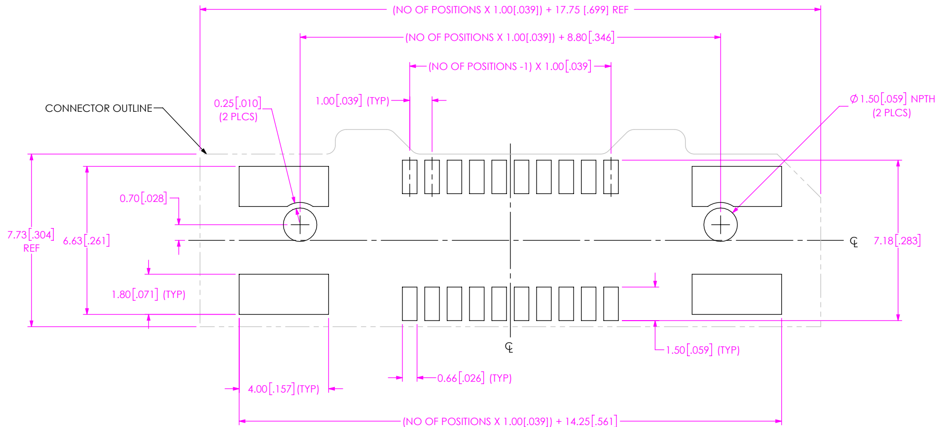
FIG 1 (-10 POSITION SHOWN) (P1M-XX-01-XXX-DV-X PCB LAYOUT SHOWN) ALL DIMENSIONS ARE SYMMETRIC ABOUT THE CENTERLINE
