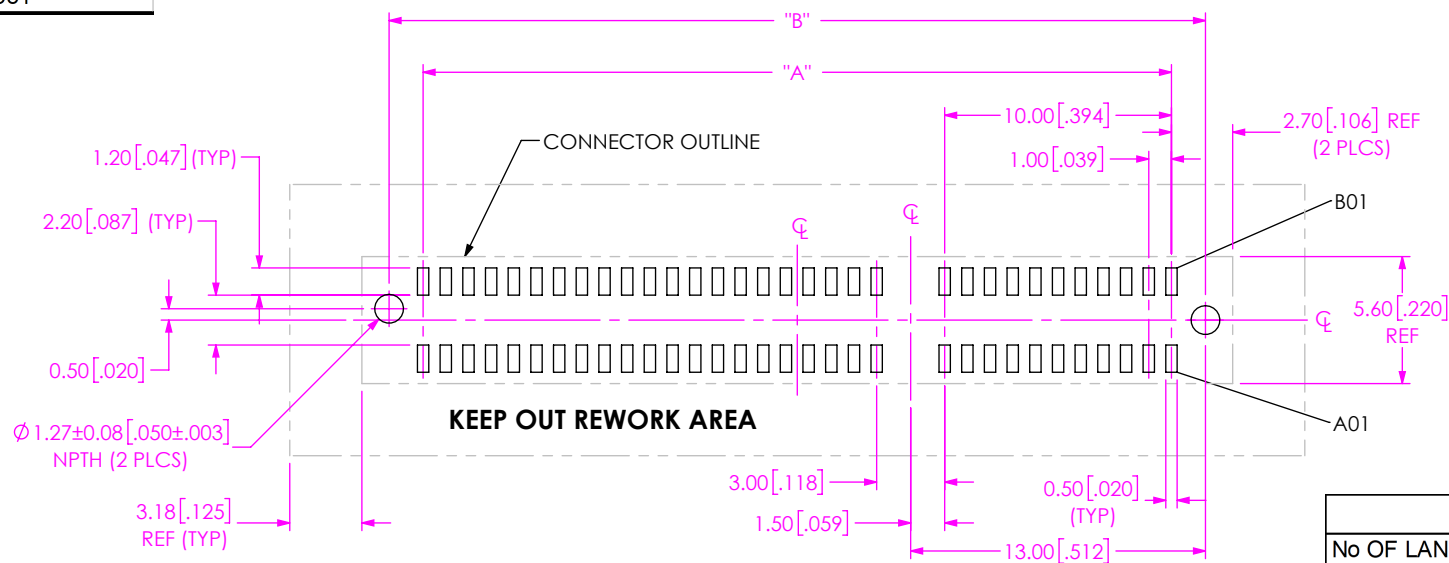
FIG 1 PCIE-G5-04-01-X-DP-A FOOTPRINT SHOWN
