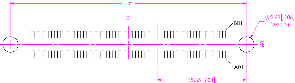
FIG 4 PCIE-G5-04-01-X-DP-A-WT STENCIL SHOWN (DIFFERENT AS SHOWN, OTHERWISE SAME AS FIG 1 & FIG 3)
