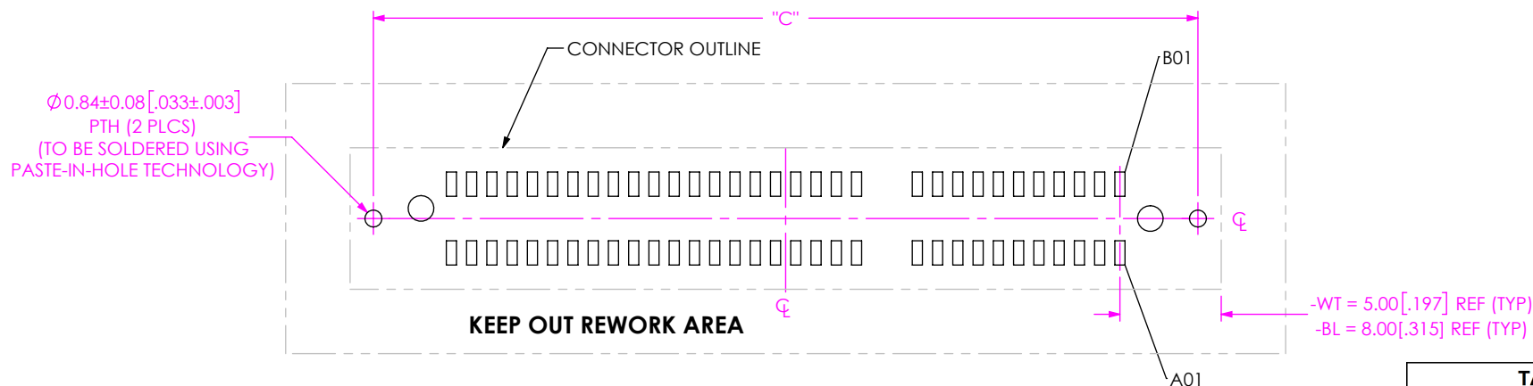
FIG 2 PCIE-G5-04-01-X-DP-A-WT FOOTPRINT SHOWN (DIFFERENT AS SHOWN, OTHERWISE SAME AS FIG 1)
