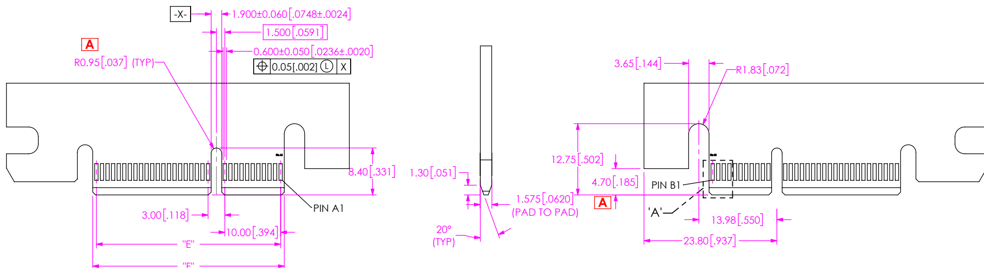
FIG 5 PCIE-G5-04-01-X-DP-A-WT MATING CARD SHOWN
