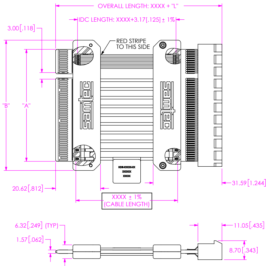
FIG 1 PCIEC-G4-098-XXXX-M1 SHOWN
