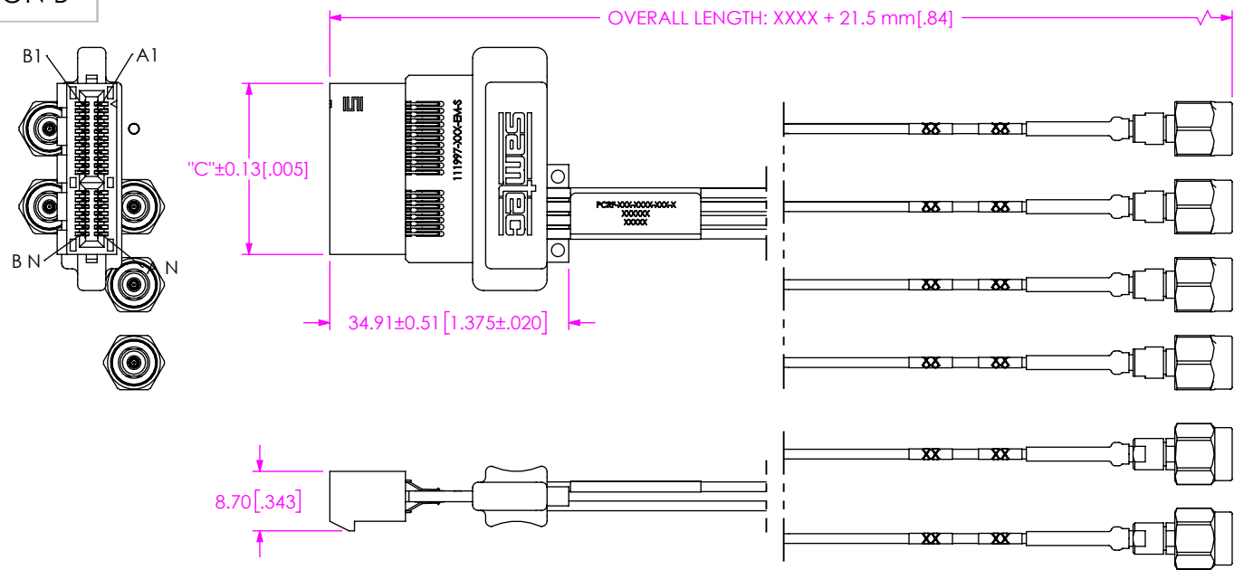
FIG 2 -EM OPTION PCR-F-G4-036-XXXX-EM-292-P-1 SHOWN (DIFFERENT AS SHOWN, OTHERWISE SAME AS FIG 1)
