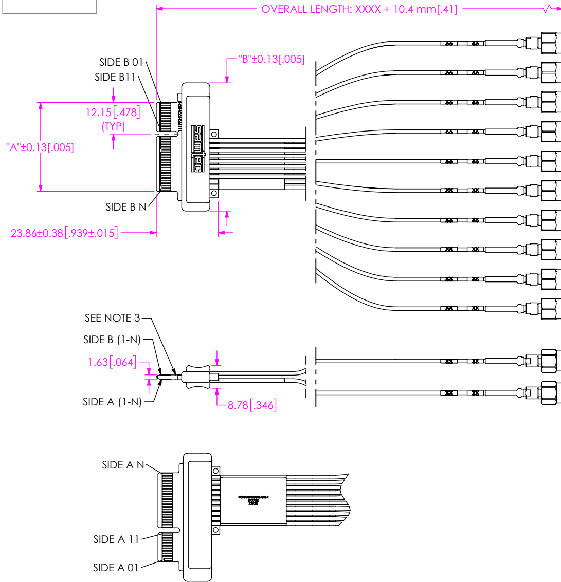
FIG 1 (PCRF-G4-064-XXXX-EC-292-P-1 SHOWN)
