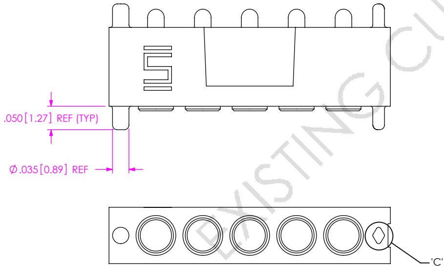
FIG. 3 PGP-05-01-G-S-AD SHOWN (SAME AS FIG. 1 EXCEPT AS SHOWN)
